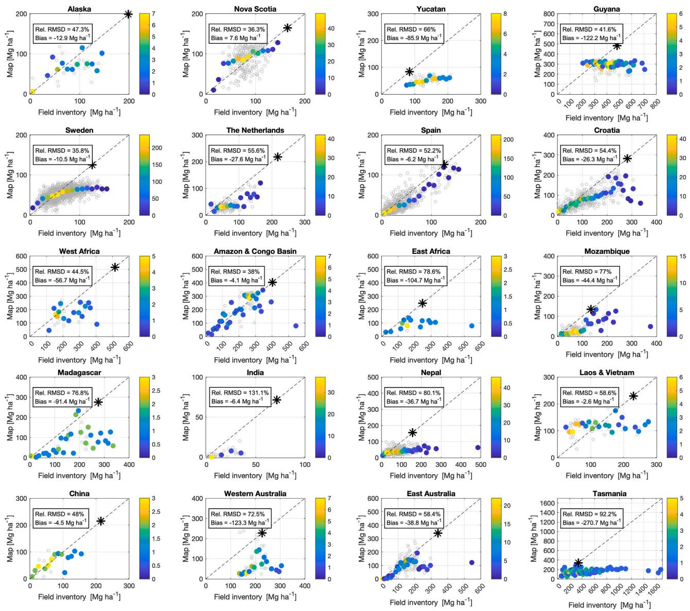
Fig. 18. Comparisons between map-based and plot-based AGB values for Tier 1 plot data spatially averaged to 0.1^\circ (grey circles). The data are grouped per region (see Fig. S13). In each panel, the map-based AGBs were also binned over 10 \text{ Mg ha}^{-1} wide ranges with filled circles representing the median mapped AGB per bin. The color bars represent the number of grid cells within a given AGB interval. Each panel includes the root mean square difference (RMSD) between map and field inventory AGB relative to the mean value of the reference AGB and the bias, i.e. the difference between mean values of the map AGB and the reference AGB. The asterisks on the identity line represent the maximum AGB in each region. (For interpretation of the references to color in this figure legend, the reader is referred to the Web version of this article.)
