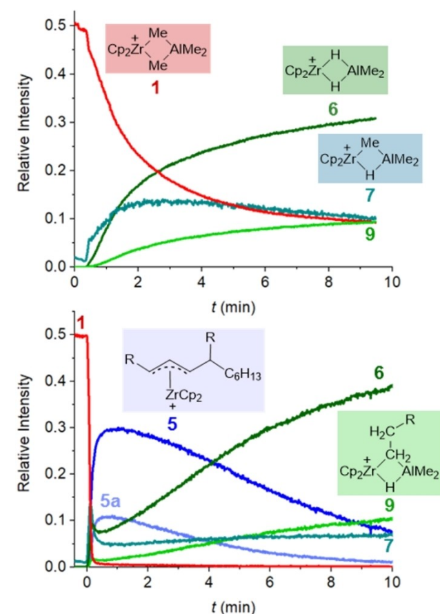
Figure 15. Normalized ion intensities vs. time for addition of (top) 10 equivalents, and (bottom) 1000 equivalents of hexene to [Cp_2ZrMe_2AlMe_2][B(C_6F_5)_4] in difluorobenzene solution with [Zr]=0.28\text{ mM} ; R='Bu . Adapted with permission from Ref. [86]. Copyright 2020, American Chemical Society.
