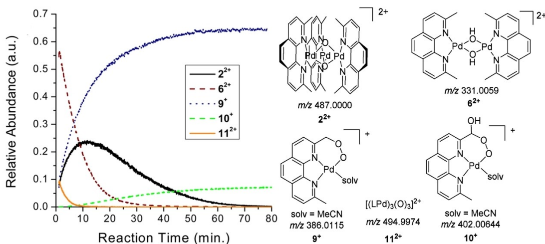
Figure 13. Left: PSI-ESI-MS monitoring of an H 2 O 2 disproportionation reaction with [(LPd(OAc)) 2 (OTf) 2 ] (L = 2,9-dimethyl-1,10-phenanthroline). Right: proposed structures of speciation. Adapted with permission from Ref. [80]. Copyright 2015, American Chemical Society.
