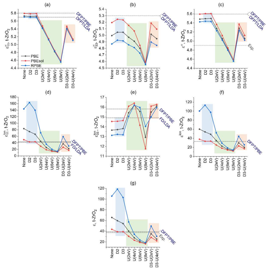
Figure 8. Electronic (a and b, \epsilon_{11}^{e} and \epsilon_{33}^{e} ) and ionic (d and e, \epsilon_{11}^{ion} and \epsilon_{33}^{ion} ) contributions to the dielectric tensor, total electronic (c, \epsilon^{e} ) and ionic contributions (f, \epsilon^{ion} ), and total dielectric constant (g, \epsilon ) of t-ZrO 2 . Previously reported experimental 9,63,64 theoretical (DFPT/LDA, DFPT/PBE, and FD/LDA) 9,18,61,62 are presented for comparison. See Table S7 (Supplementary Material).
