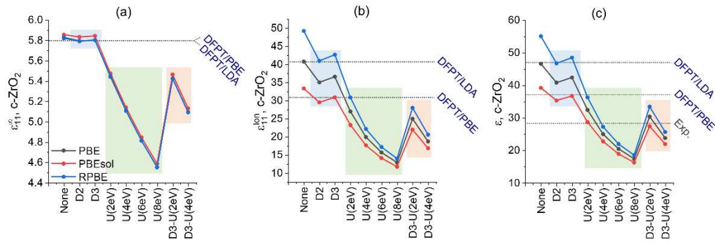
Figure 7. Electronic (a, \epsilon_{11}^{e} ) and ionic (b, \epsilon_{11}^{ion} ) contributions to the dielectric tensor, and total dielectric constant (c, \epsilon ) of c-ZrO 2 . Previously reported experimental 9,63,64 and theoretical (DFPT/LDA and DFPT/PBE) 9,61,62 values are presented for comparison. See Table S6 (Supplementary Material).
