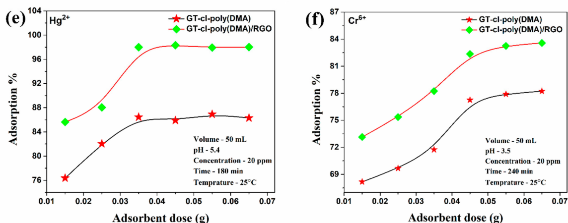
Figure 6. Influence of (a) RGO loading on Hg 2+ adsorption (b) RGO loading on Cr 6+ adsorption, (c) pH on adsorption of Hg 2+ , (d) pH on adsorption of Cr 6+ , (e) adsorbent dose on adsorption of Hg 2+ , (f) adsorbent dose on adsorption of Cr 6+ . Adsorbent: gum tragacanth- cl-N,N -dimethylacrylamide (GT- cl-poly (DMA)) hydrogel and reduced graphene oxide incorporated gum tragacanth- cl-N,N -dimethylacrylamide (GT- cl-poly (DMA)/RGO) hydrogel composite.
