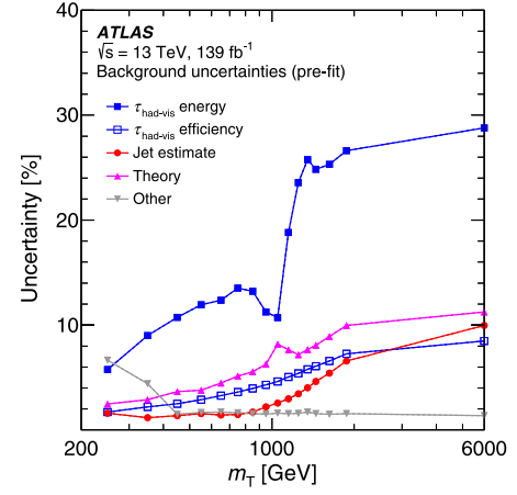
FIG. 5. Relative systematic uncertainties (in %) on the total background yield before the likelihood fit to data ( prefit ) as a function of m_T . The filled squares show the uncertainty due to the \tau -lepton energy scale, the open squares show the uncertainties originating from the \tau -lepton reconstruction and identification efficiencies, the circles show the uncertainty originating from the jet background estimation, and the upward triangles show the uncertainty from the simulated background cross sections. Additional sources of uncertainty, such as those from the trigger efficiency measurement, the jet energy scale and the luminosity, are combined in the downward arrows.
