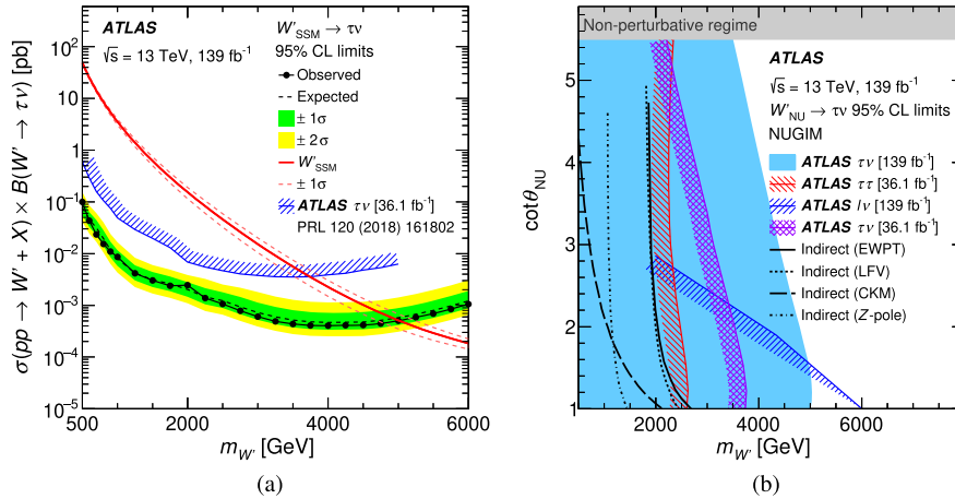
FIG. 7. (a) Observed (black markers) and expected (black dashed line) 95% CL upper limits on the cross section times branching ratio ( \sigma \times B ) as a function of the W' mass in the SSM. The inner and outer bands show the \pm 1 and \pm 2 standard deviations, respectively, of the expected limit. The solid red line represents the theoretical cross section and the dashed red lines represent its theoretical uncertainty for the SSM signal. The blue hatched line indicates the observed 95% CL upper limits on \sigma \times B of the previous ATLAS \tau\nu [10] search. (b) Observed 95% CL lower limit on the W' mass as a function of the parameter \cot\theta_{\text{NU}} describing the coupling to the third generation. The blue shaded area represents the exclusion limits set by this analysis of the full run 2 data sample of ATLAS. For the same data sample, the exclusion limits set by the W' \rightarrow \ell\nu search [9] are also shown as blue forward hatched line. The observed limits from the previous ATLAS \tau\nu [10] (purple diagonal crosses) and \tau\tau [71] (red backward hatched line) searches with 36.1 \text{ fb}^{-1} are overlaid for comparison. The W' and Z' bosons are assumed to be degenerate in mass. Indirect limits at 95% CL from fits to electroweak precision measurements (EWPT) [12], lepton flavor violation (LFV) [13], CKM unitarity [14] and the Z-pole data [2] are also overlaid.
