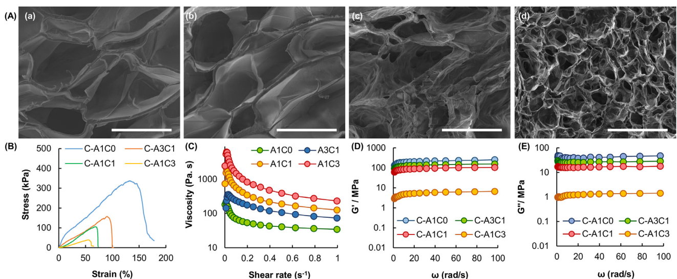
Fig. 3 – (A) SEM micrographs of the cross-sections of complex fibers consisting of (a) C-A1C0, (b) C-A3C1, (c) C-A1C1, and (d) C-A1C3. Scale bar = 500 µm. (B) Tensile stress-strain curves of different complex fibers. (C) The viscosity of different Na-Alg/CMC-Na blends at shear rates from 0 to 1 s -1 . (D) The G' values and (E) G'' values of different complex fibers at angular frequencies from 0.1 to 100 rad/s.
