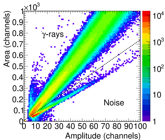
Fig. 9. 2D plot showing the amplitude versus the area of the sTED signals with an R11265U-100 photomultiplier when measuring an ^{88}\text{Y} calibration source. The black dashed line separates two different types of signals, see text for details. The bottom figure is a zoom of the top one.
