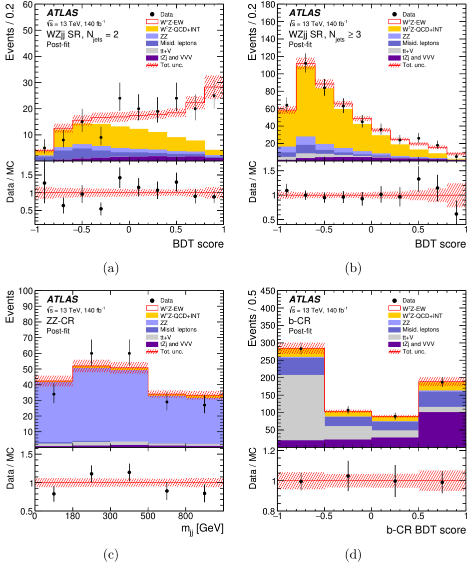
Figure 3. Post-fit distributions of (a) the BDT score distribution in the signal region, for N_{jets} = 2 and (b) N_{jets} \geq 3 categories, (c) m_{jj} in the ZZ-CR control region, (d) the b -CR BDT score in the b -CR. Signal and backgrounds are normalised to the expected number of events after the fit. The uncertainty band around the MC expectation includes all systematic uncertainties as obtained from the fit.
