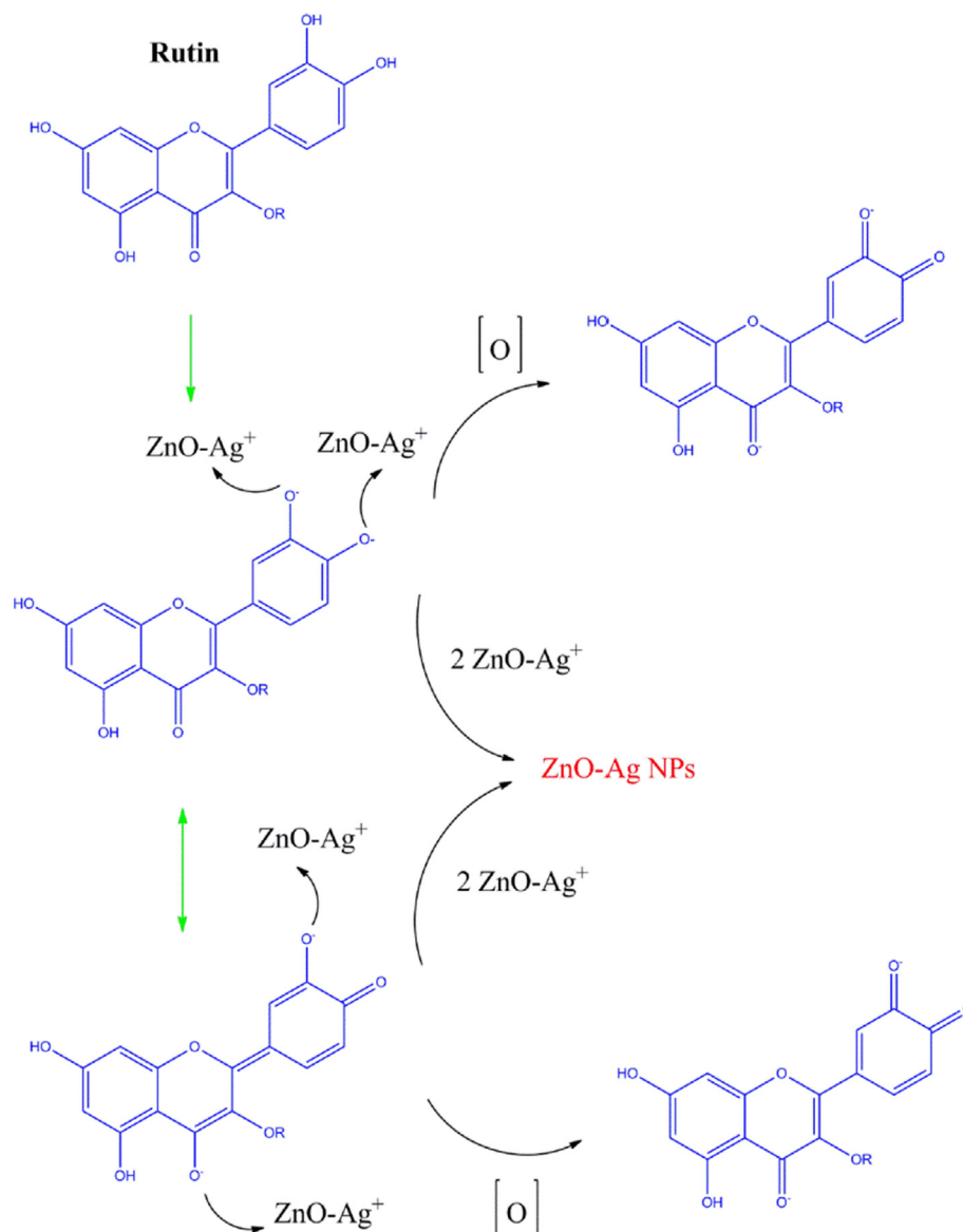
Fig. 1 The possible mechanism of the bio-synthesis of ZnO-Ag using C. monogyna extract.
