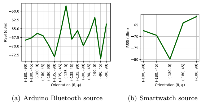
Fig. 19. Sensitivity of the Bluetooth RSSI to the device orientation in an office environment. We observe a large variability of the RSSI with the device orientation for both sources.
