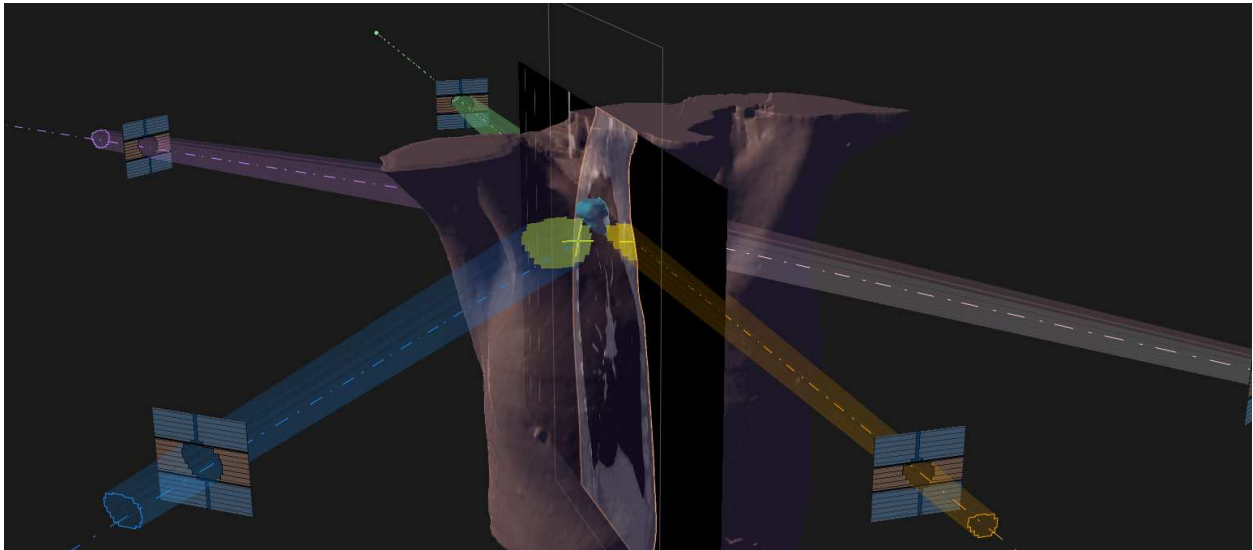
Figure 3. Computer systems help design radiotherapy treatments in which multiple beams are angled around the patient, each beam being shaped to match to the target.
