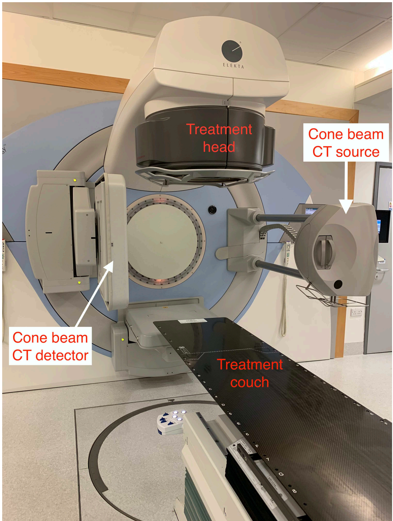
Figure 1. Linac with cone-beam CT equipment at right angles to the treatment head. Figure from Elekta with permission.
