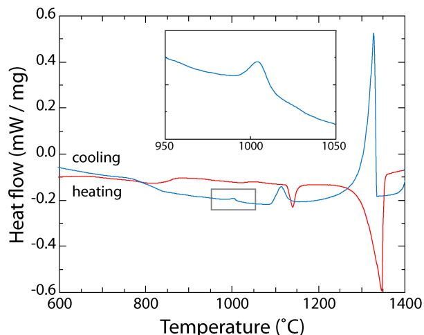
2 DSC thermogram from as cast Al 0.5 CrFeCoNiCu during heating (red) and cooling (blue) at 10°C min -1
