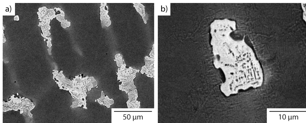
3 BSEI micrographs (a 50 μm; b 10 μm) of Al 0.5 CrFeCoNiCu cooled at 10°C min -1 from the liquid state
