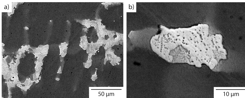
7 BSEI micrographs (a 50\ \mu\text{m} , b 10\ \mu\text{m} ) of \text{Al}_{0.5}\text{CrFeCoNiCu} cooled at 50^\circ\text{C min}^{-1} from the liquid state
