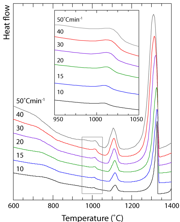
6 DSC thermograms illustrating the influence of cooling rate on \text{Al}_{0.5}\text{CrFeCoNiCu}
