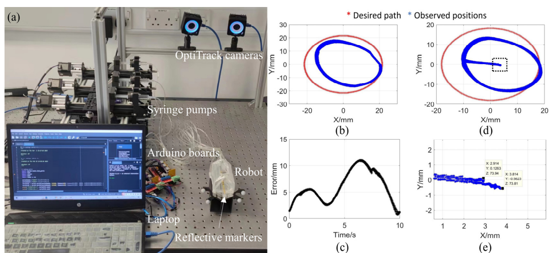
Figure 16. Robot tracking. (a) The test setup. (b) The results of tracking a 43 mm diameter circle. (c) The tracking errors. (d) The results of tracking a 36 mm diameter circle. (e) An enlarged view around the initial point.
