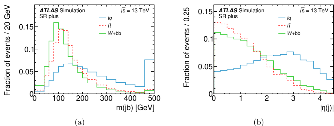
Figure 2. Probability densities of the two most discriminating input variables to the NN in SR plus . (a) The invariant mass m(jb) of the untagged jet and the b -tagged jet and (b) the absolute value of the pseudorapidity of the untagged jet |\eta(j)| . The distributions are shown for the tq signal process, and the t\bar{t} and the W+b\bar{b} backgrounds. Events beyond the x -axis range are included in the last bin.
