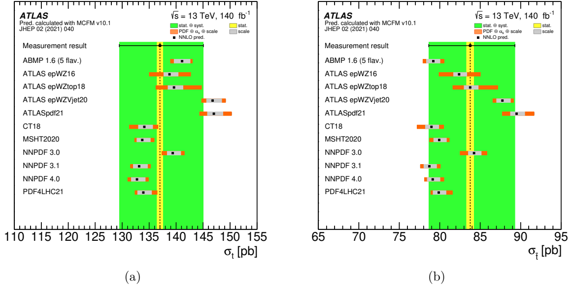
Figure 13. Comparison of NNLO predictions based on several different PDF sets with the measured values (dots) of (a) \sigma(tq) and (b) \sigma(tT) . The yellow band represents the statistical uncertainty and the green band the total uncertainty. The uncertainties in the theoretical predictions include PDF, scale and \alpha_s uncertainties.
