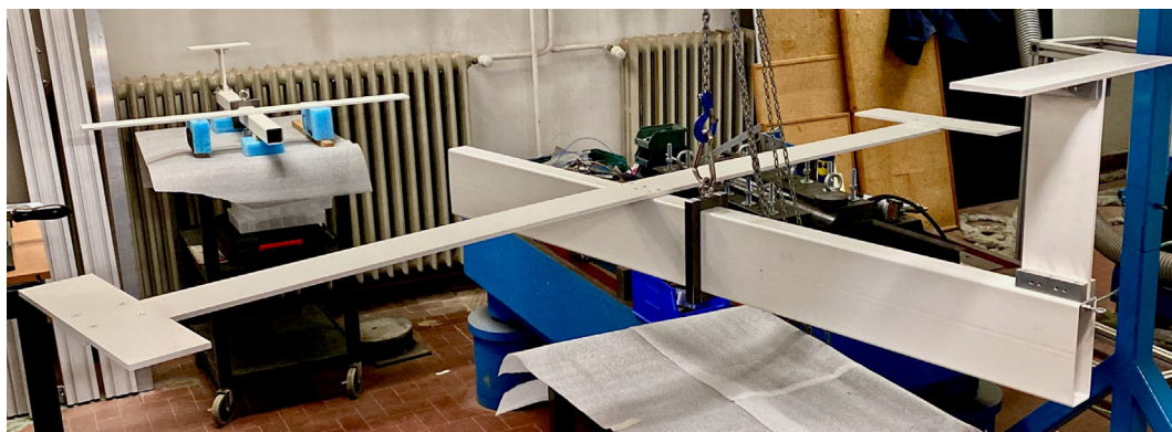
FIGURE 2 Garteau laboratory-scale model.
