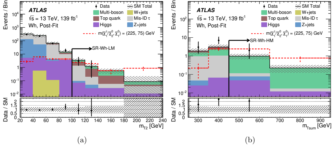
Figure 15. The kinematic distributions for the Intermediate Wh channel after the background-only fit, showing (a) m_{T2} in SR-Wh-LM and (b) m_{T\text{sum}} in SR-Wh-HM, before the selection on that kinematic is made. The black arrow depicts the selection for the signal region. An example SUSY scenario is overlaid for illustration. The hashed bands represent the combined statistical and systematic uncertainties of the total SM background. The lower panels show the ratio of data to the total SM background estimate.
