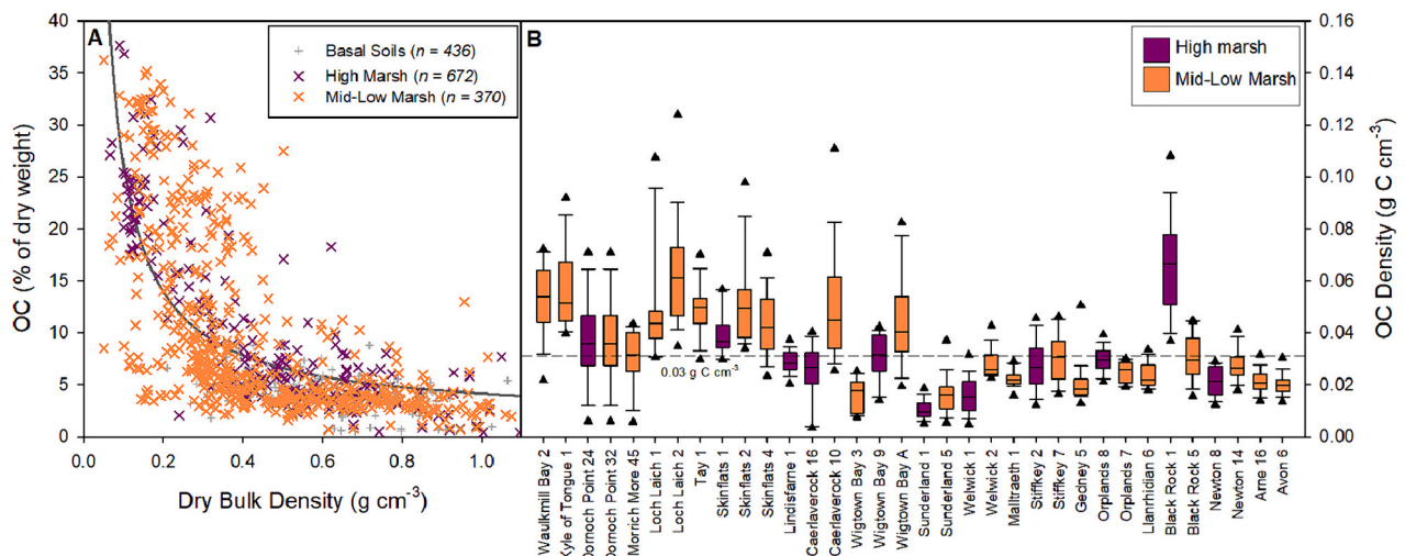
Fig. 3. Organic carbon density of Great British saltmarsh sediments. (A) Dry bulk density vs organic carbon (OC) content. Black line reflects the correlation ( y = 2.3874 \times 10^{-53} ) between the dry bulk density and OC (%). (B) Centimetre-resolution OC density ( \text{g C cm}^{-3} ) of the saltmarsh cores (core identification along the x-axis) arranged by latitude (furthest north on the left-hand side). The solid line within the boxes represents the median value, and the triangles illustrate the 5th and 95th percentiles. The black dashed line represents the mean OC density calculated from all cores in this study. Supplementary Fig. 28 displays downcore OC content records for all 34 cores.
