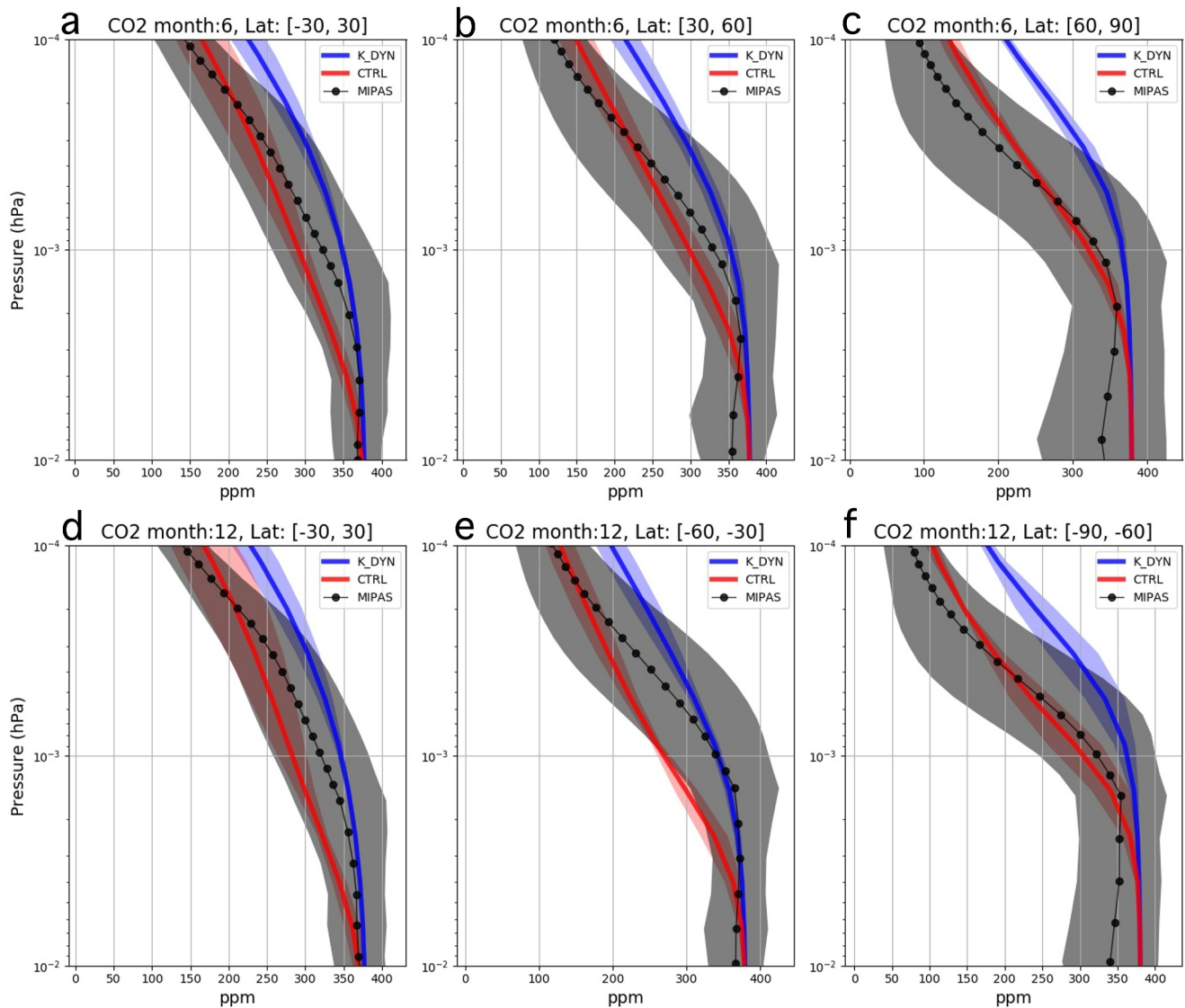
Figure 11. Vertical profiles of CO 2 mixing ratio for June in the Northern Hemisphere (a, b, c) and December in the Southern Hemisphere (d, e, f) (i.e., summer solstice conditions) for MIPAS observations (black dots), K_DYN (blue line) and CTRL (red line) for years 2008–2011. Area-weighted means were computed over the tropics (a, d), mid-latitudes (b, e) and polar regions (c, f). Shaded areas correspond to two times the standard deviation of the spatial mean for both modeled and observed data.
