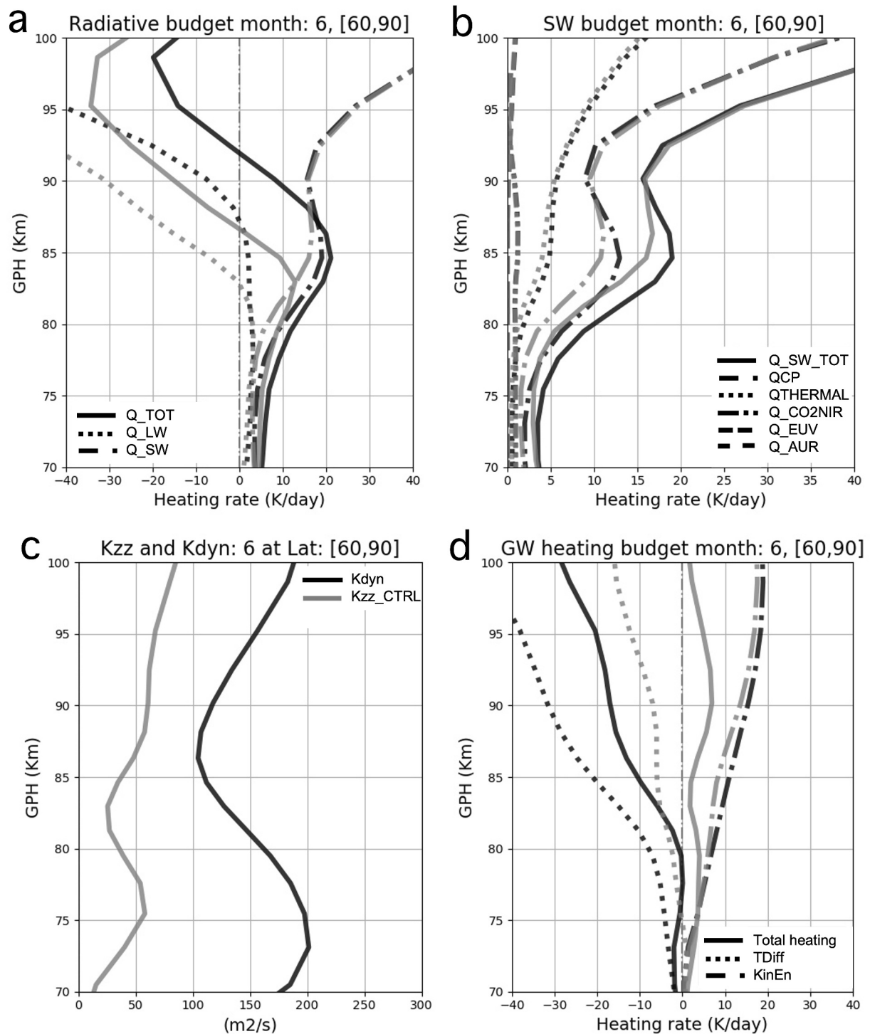
Figure 10. Vertical profiles of total radiative heating budget (a), short-wave radiation budget (b), K_{zz\_CTRL} and K_{D_{dyn}} (c), and gravity wave heating budget (d) for K\_DYN (black line) and CTRL (gray line) for Northern Hemisphere summer conditions (June) between 60^\circ N and 90^\circ N .
