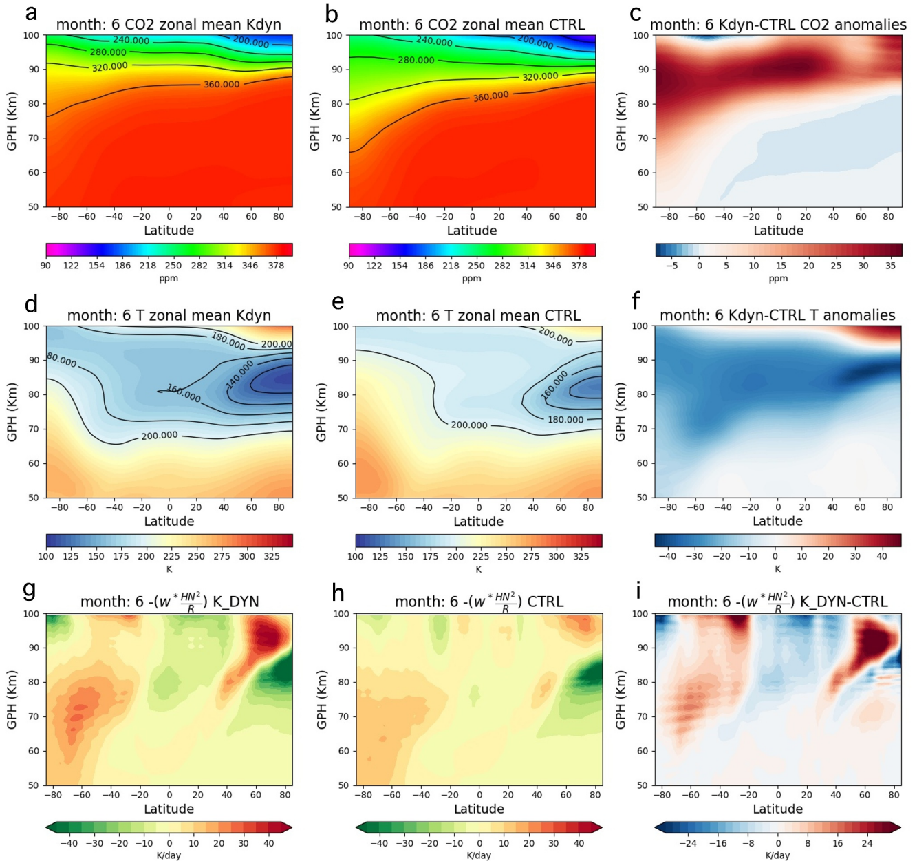
Figure 7. Zonal mean cross-sections of CO 2 mixing ratio, air temperature (T), and expected temperature departure from radiative equilibrium ( -w^* \left( \frac{HN^2}{R} \right) ) as simulated by K_DYN (a, d, g), CTRL (b, e, h) and their difference (c, f, i) for Northern Hemisphere summer conditions (June).
