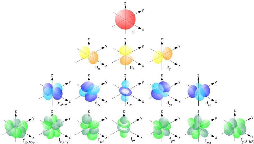
Figure 2. The Exclusion Principle restricts how many electrons can occupy an energy state, giving nested orbitals. Credit: Wikimedia Commons.
