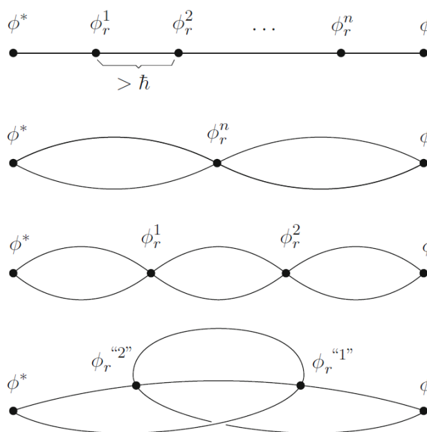
Figure 3. The many-instant landscape, in which causal ordering and temporal ordering can come apart. Image: Henrique Gomes, reproduced from [6].
