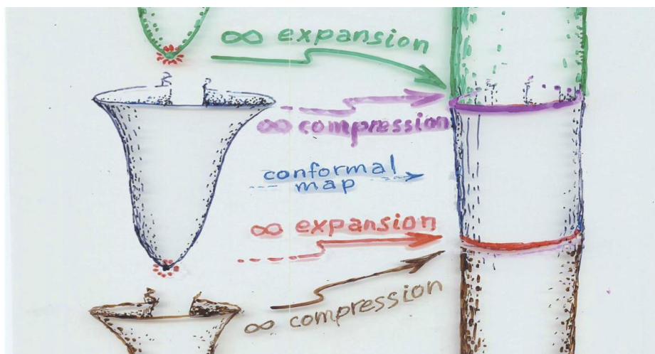
Figure 4. In conformal cyclic cosmology, the death of one spacetime is the birth of another. Credit: Roger Penrose.
