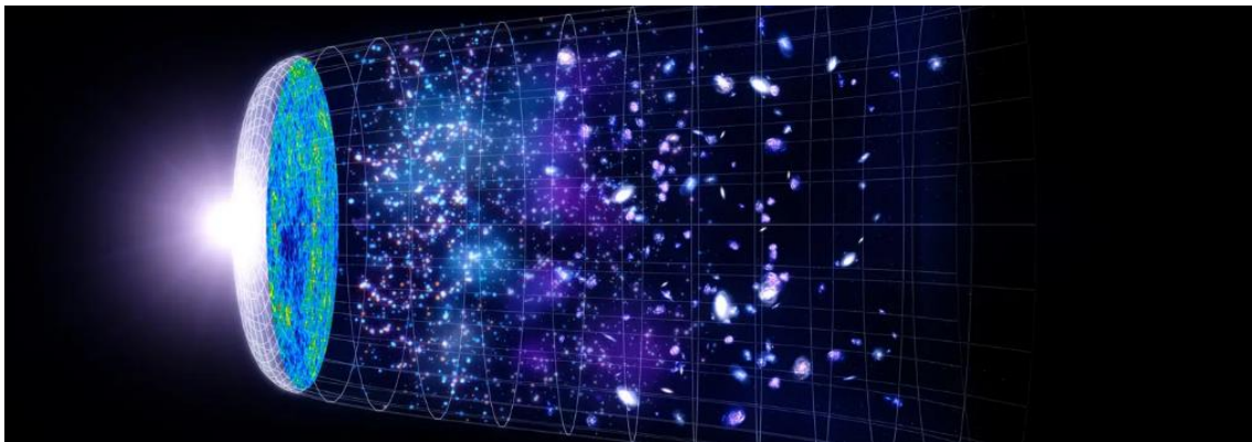
Figure 1. All spacetime trajectories approach the Big Bang. Credit: NASA.
