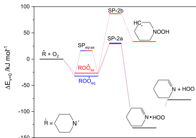
Figure 4. Relative energies of stationary points on the potential energy surface relevant to the 1-piperidinyl radical reaction with O 2 . Results from CCSD(T*)-F12a/aug-cc-pVTZ//M062X/aug-cc-pVTZ calculations. The underlying quantum chemistry data are summarized in Table S8.
