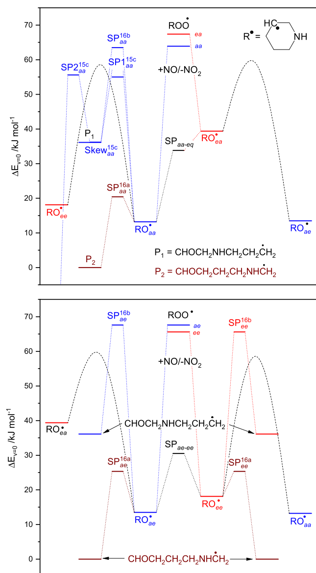
Figure 9. Stationary points on the potential energy surface relevant to the unimolecular reactions of the 3-piperidinyl oxy radical, PIP 3 O. For the sake of simplicity, the high-barrier 1,4-H transfer reactions 15a and 15b have not been included in the figure. Top: ea and aa manifold. Bottom: ae and ee manifold. The dashed curves mimic the complicated conformational links between the ea and ae and the ee and aa conformers. Results from CCSD(T*)-F12a/aug-cc-pVTZ//M062X/aug-cc-pVTZ calculations. The underlying quantum chemistry data are collected in Table S13.
