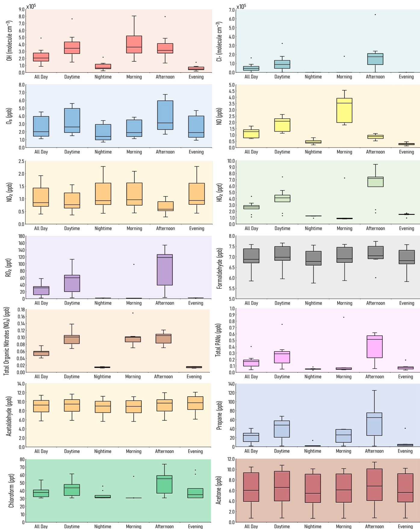
Fig. 3 Concentrations of key indoor species from ten different houses, showing the median, the upper (75%) and lower (25%) percentiles and the upper ( Q3 + 1.5 \cdot IQR ) and lower whiskers ( Q1 - 1.5 \cdot IQR ). The small circles represent values which lie outside of the upper and lower whisker range. The denoted time periods are: all day (12am to 12am), daytime (7am to 7pm), nighttime (7pm to 7am), morning (6am to 12pm), afternoon (12pm to 6pm) and evening (6pm to 10pm).
