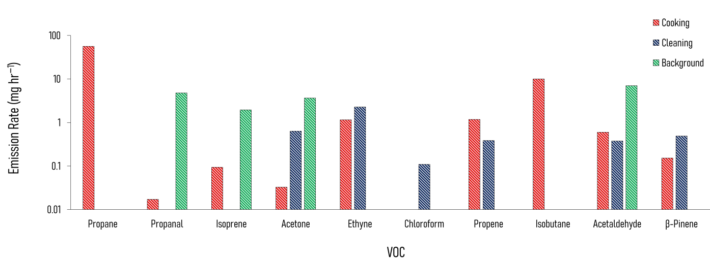
Fig. 4 The enhancement in emission rates from indoors to outdoors over background values for a variety of VOCs ( \text{mg hr}^{-1} ) during cooking and cleaning, from the house described in Section 2.4.1. The background emission rates are shown for comparison, and comprise of emissions from building and furnishing materials and from people.
