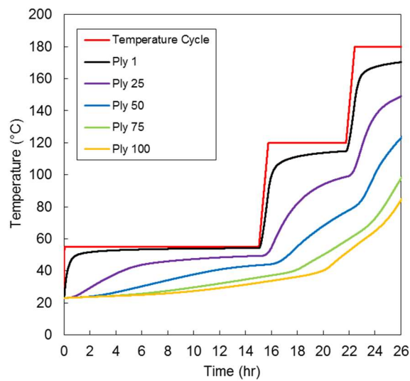
4 Figure A.6. Simulated temperatures in a 100-ply laminate manufactured using a heated steel tool, and 200 5 mm insulation at the top boundary. The laminate consisted of UD GF and epoxy powder (GRN 918).
