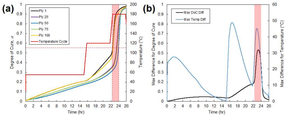
19 Figure 15. (a) Simulated DoC evolution for the 100-ply laminate of UD GF/GRN 918. The horizontal 20 dashed red line represents the gel point ( \alpha_g = 0.56 [12]), while the shaded red area shows the timespan of 21 gelation in the laminate. (b) Plot of the maximum DoC difference and the maximum temperature 22 difference. The peaks in the max differences overlap with gelation of the laminate, meaning that any corresponding residual stresses would be locked in.
