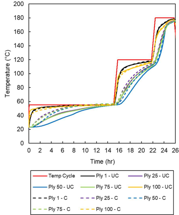
1 2 Figure 13. Comparison of simulations for a consolidated (C) laminate and an unconsolidated (UC) 3 laminate. The consolidated laminate simulation assumed a constant thickness throughout.
