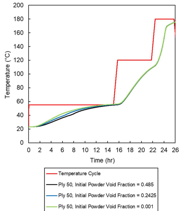
2 Figure 12. Plot of the temperature at Ply 50 for varying levels of initial powder void fraction.
