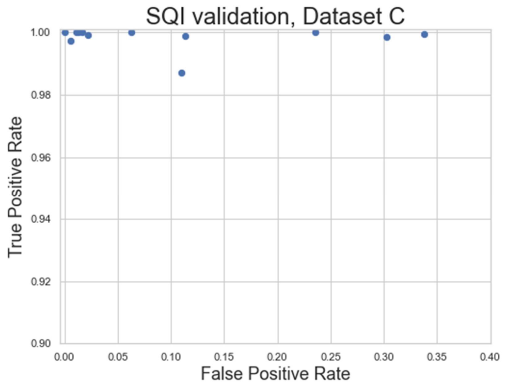
Figure 14. A demonstration of the SQI algorithm on a noisy dataset. Each dot represents one recording. The algorithm has a very good true positive rate (sensitivity), but a slightly worse false positive rate (1-specificity), implying it will often identify good areas, but may not reject areas of bad HR as often as it should.
