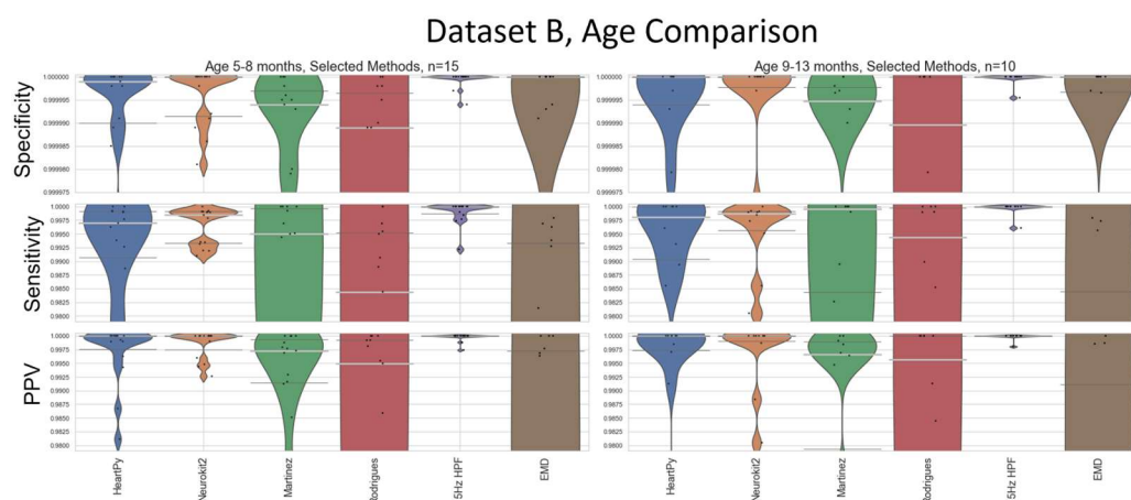
Figure A2. An age-based breakdown of Figure 9. A different age bracket is shown in each quadrant. The median is shown as a thick, light grey bar, and the IQR is shown as thin dark grey bars. Each black dot represents one result.
