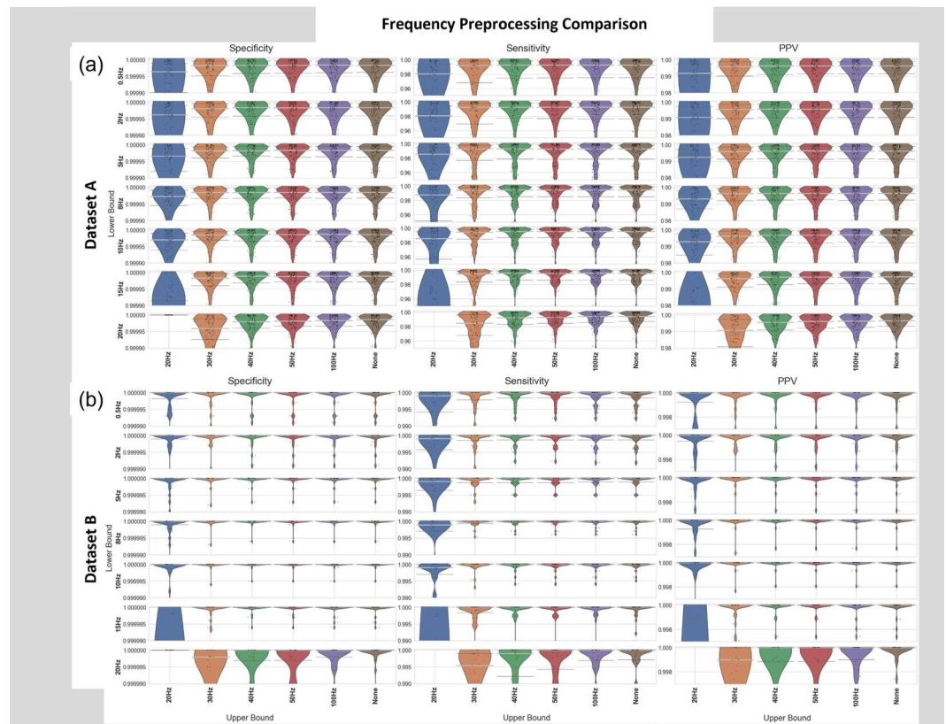
Figure 7. The Specificity, Sensitivity, and PPV (columns 1, 2, and 3) results shown as violin plots for a selection of frequency-preprocessing methods applied to (a) Dataset A, and (b) Dataset B. In all subplots, the median is shown as a thick, light grey bar, and the IQR is shown as thin dark grey bars. Each black dot represents one result. The lower frequency bounds are shown on the y-axis, the upper frequency bounds on the x-axis (with the right-most column of each subplot indicating no upper bound, i.e., an HPF). Results are all shown at a consistent scale, violin plots which go to the edge of the graph may have results outside the visualized range.
