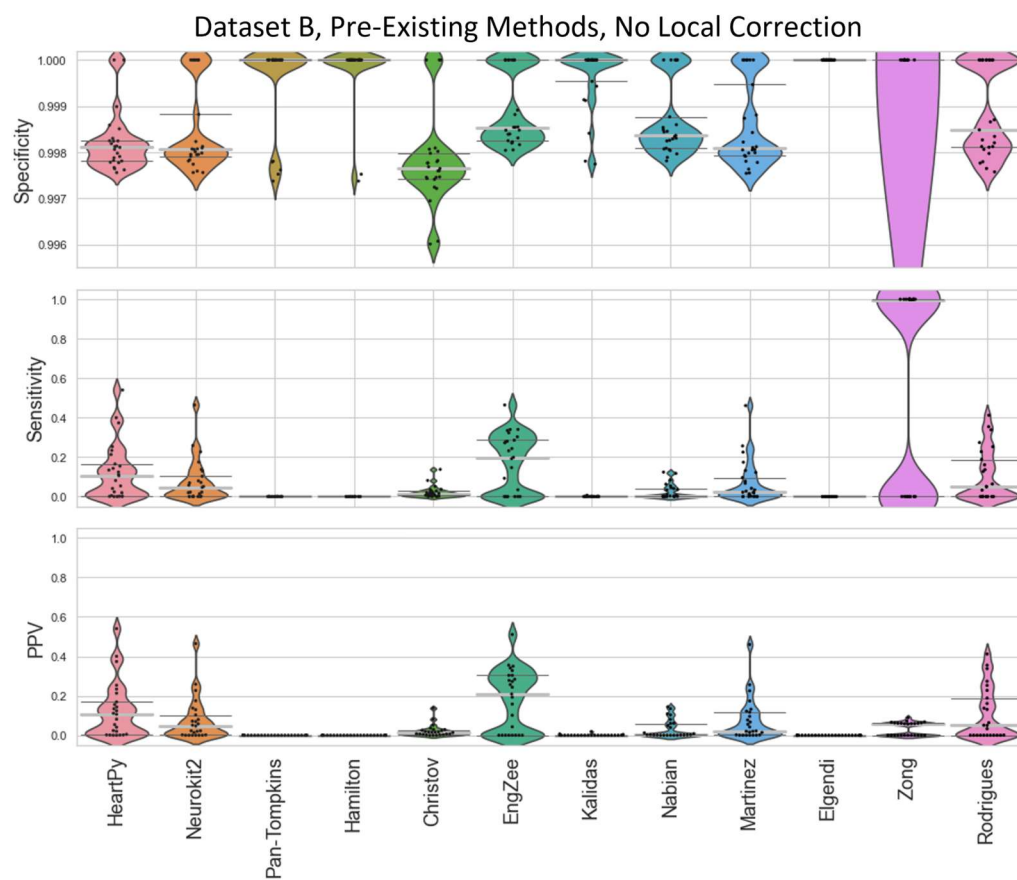
Figure A4. Violin plots showing the specificity, sensitivity, and positive predictive values for the pre-existing ECG approaches applied to Dataset B, with no local peak correction.
