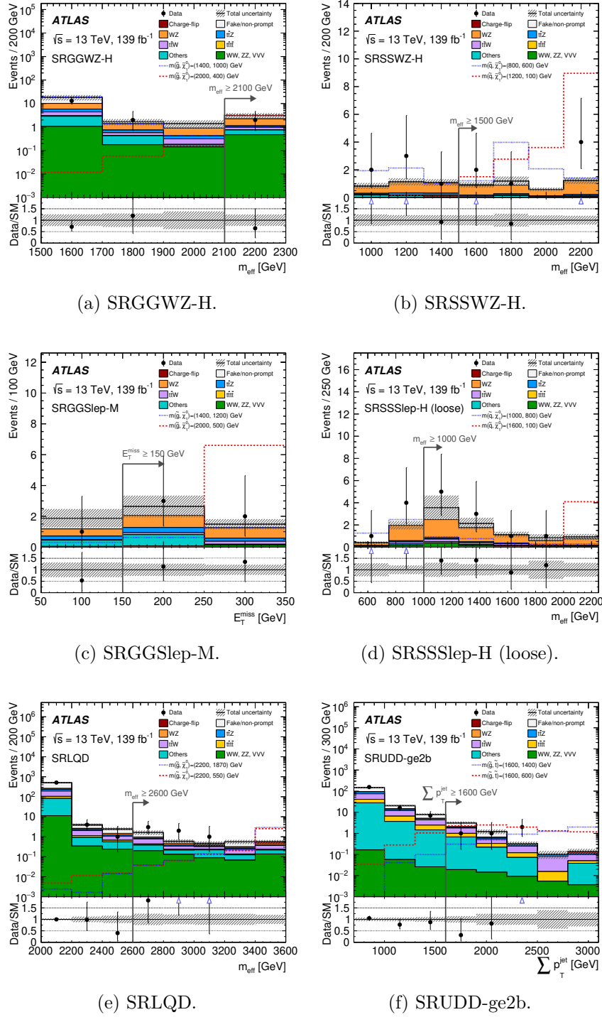
Figure 6. Distributions of the data and estimated background after the background-only fit for the signal regions (a) SRGGWZ-H, (b) SRSSWZ-H, (c) SRGGSlep-M, (d) SRSSSlep-H (loose), (e) SRLQD, and (f) SRUDD-ge2b. All SR selections but the one on the quantity shown are applied. The line with an arrow indicates the requirement used in that signal region. Distributions for two signal hypotheses for the model of interest are also shown. The bins displayed above the signal region requirement correspond to the binning used in the exclusion fit. All uncertainties are included in the uncertainty band. Overflow (underflow) events, where present, are included in the last (first) bin.
