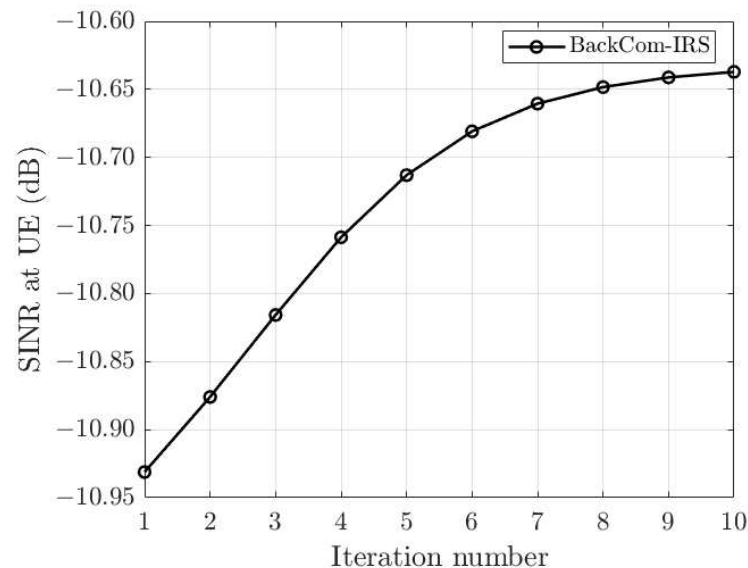
Figure 2. Convergence of the BackCom-IRS scheme in a random observation.
