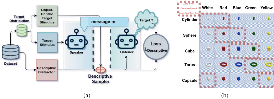
Figure 1: (a): Illustration of a descriptive object-centric (partially-observable) 2-players/L-signal/N = 0-round/K = 0-distractor referential game . (b): Example images of the dataset showing the different objects (in specific viewpoints), along with a possible zero-shot compositional learning train-test split example.
