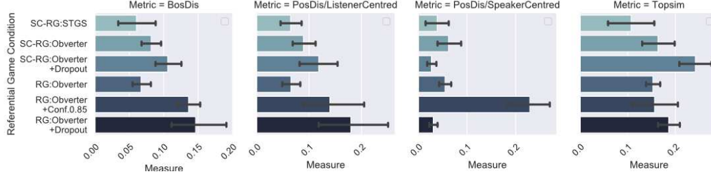
Figure 3: Compositionality metrics for the different referential game approaches, at the end of training.
