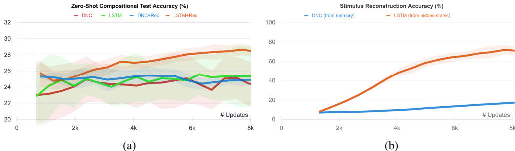
Figure 6: (a) : 4-ways (3 distractors) zero-shot compositional test accuracies of different architectures. 5 seeds for architectures with DNC and LSTM, and 2 seeds for runs with DNC+Rec and LSTM+Rec, where the auxiliary reconstruction loss is used. (b) : Stimulus reconstruction accuracies for the architecture augmented with the auxiliary reconstruction task. Accuracies are computed on binary values corresponding to each stimulus’ latent dimension’s reconstructed value being close enough to the ground truth value, with a threshold of 0.05.
