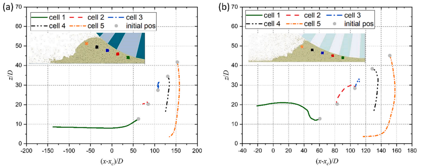
Fig. 10. Averaged trajectories of the particles in five tracking cells for Ancor sample: (a) \omega = 4 rps and (b) \omega = 12 rps. Grey dots show the initial averaged position of the particles for each cell.
