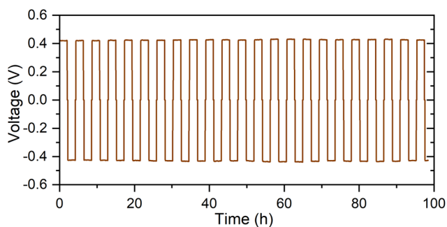
Fig. 7 Galvanostatic cycling data of a Li/ \text{Li}_4\text{P}_2\text{O}_7/\text{Li} symmetric cell at 80 \text{ }^\circ\text{C} and 2 \mu\text{A cm}^{-2} current density.
