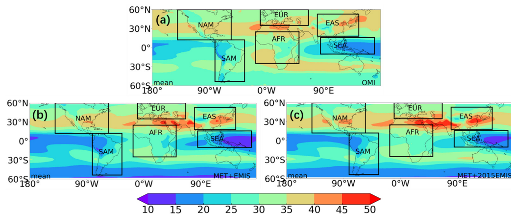
Figure 1. Multi-year mean spatial distribution of tropospheric column ozone (TCO) (DU) based on OMI/MLS satellite data ((a), 2005–2020), simulated results of case MET+EMIS ((b), 2001–2015) and case MET+2015EMIS ((c), 2001–2020).
