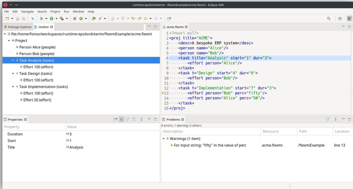
Fig. 6 The FLEXMI editor and its integration with the Outline, Properties and Problems view from the Eclipse IDE
