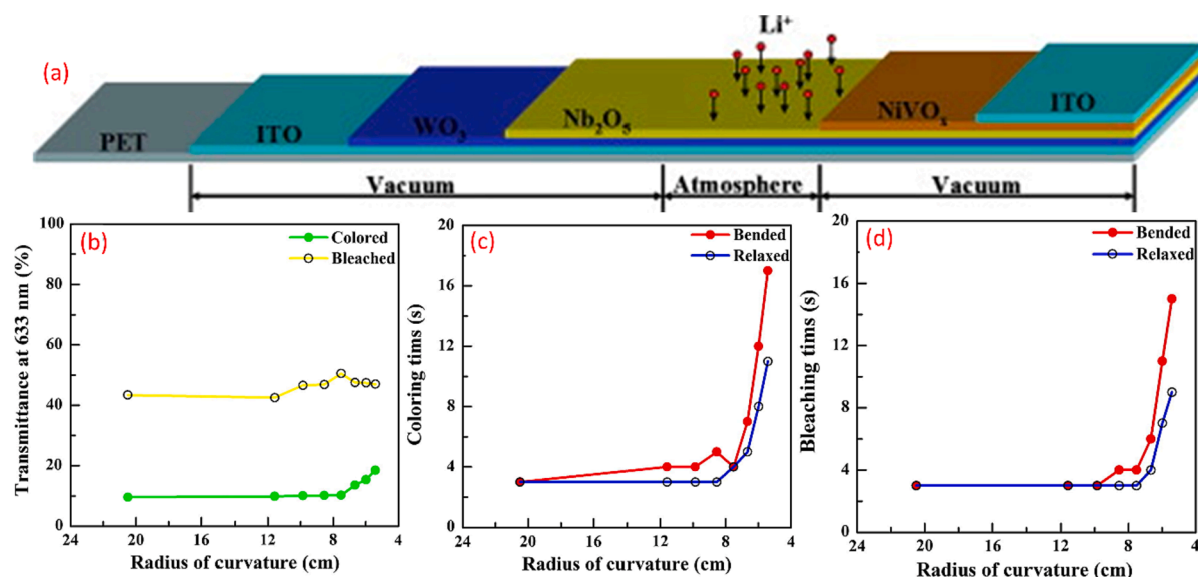
Fig. 16. (a) Layered monolithic structure of the flexible EESD constructed based on ITO/WO 3 /Nb 2 O 5 /NiVO 3 /ITO [143] and its (b) transmittance, (c) colouring time and (d) bleaching time for the 3.5 cm × 5.5 cm EESD under different radii of curvature in static bending. Reprinted from [143] Copyright (2016), with permission from Elsevier.
