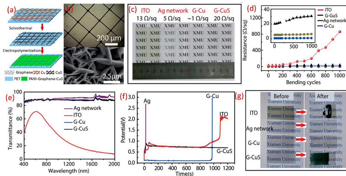
Fig. 7. (a) Solvothermal and electropolymerization reactions for synthesizing G-CuS/PANI on the PET substrate. (b) Scanning electron microscopic image of G-CuS network. Comparison of performances of various properties of G-Cu, G-CuS, Ag network and ITO transparent flexible electrodes including (c) electrical properties (d) resistance variation under mechanical bending (e) optical transmittance (f) chemical stability through chronoamperometry study and (g) deposition of PANI film via electropolymerization. (a-g) Reproduced from Ref. [51] with permission from the Royal Society of Chemistry.
