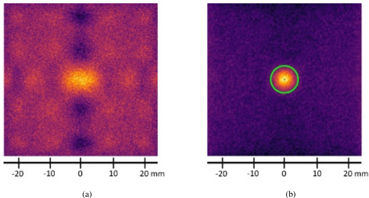
FIG. 4: a) A synthetic hologram from a P_0 of 40 \text{ m } 10^{14} yield NIF-like neutron source and (b) its reconstructed source image with \chi^2 \leq 1 and a P_0 = 43 \pm 3 \text{ m} shown in green.
