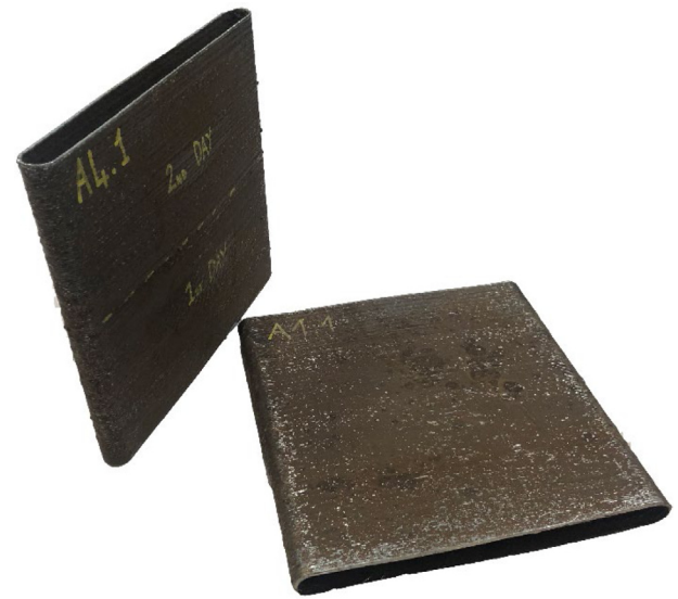
Fig. 2. WAAM oval tubes from which test specimens were cut.
