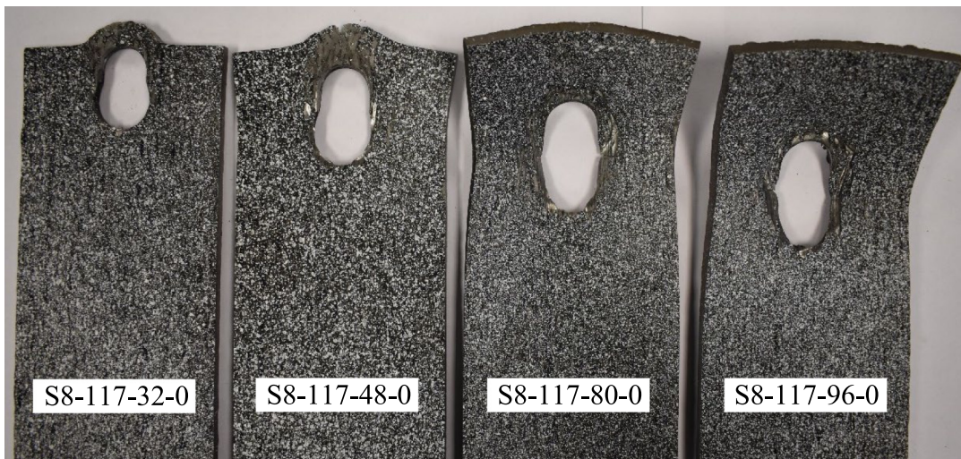
Fig. 17. Failure mode transition from shear-out to end-splitting and localised tearing failure.
