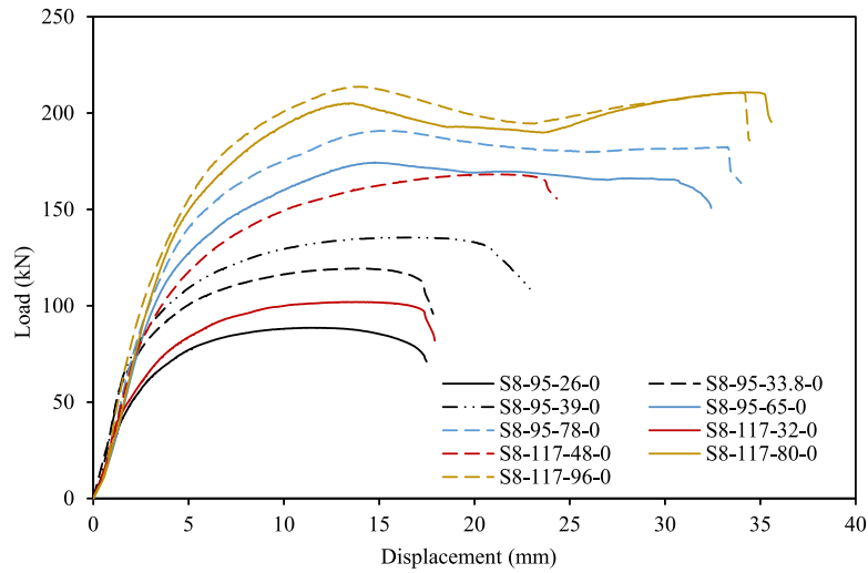
(g) t = 8 mm, \theta = 0^\circ and b varying from 95 and 117 mm
