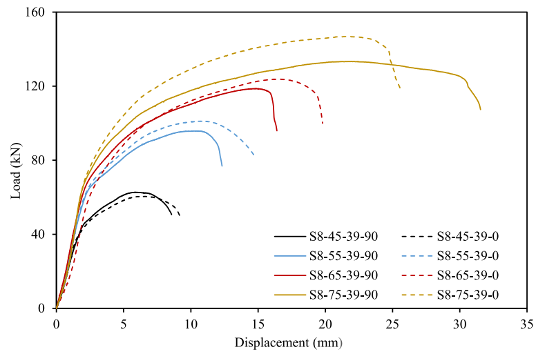
(e) t = 8 \text{ mm} , \theta = 90^\circ and l varying from 45 to 75 mm
