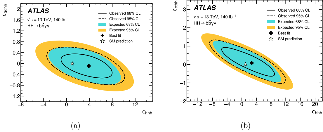
Figure 7. Likelihood contours at 68% (solid line) and 95% (dashed line) CL in the (a) c_{gghh} versus c_{hhh} and (b) c_{tthh} versus c_{hhh} HEFT parameter space, with the remaining coefficient fixed to its SM value. The corresponding expected contours are shown by the inner and outer shaded regions. The SM prediction is indicated by the star, while the best-fit value is denoted by the cross.
