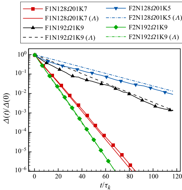
Figure 7. Comparison between the decay rates of \Delta(t) and the CLEs.
