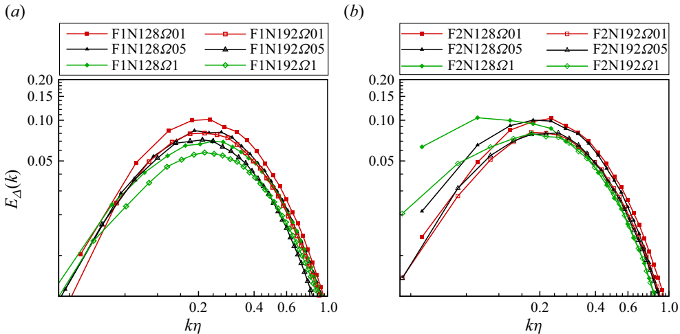
Figure 12. The energy spectra of the Lyapunov vectors \mathbf{u}^\delta for k_m = 0 : (a) for the cases with Kolmogorov forcing; (b) for the cases with constant power forcing. The spectra have been normalised in such a way that the total energy is unity.
