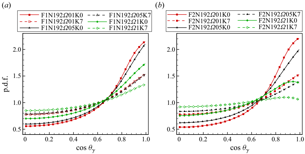
Figure 20. The p.d.f.s of \cos \theta_\gamma : (a) cases with Kolmogorov forcing; (b) cases with constant power forcing.
