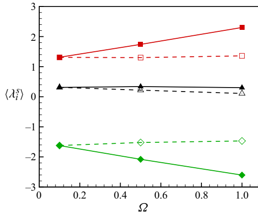
Figure 21. The mean values of the eigenvalues of the dimensionless strain rate tensor s_{ij}^+ . Solid lines indicate cases with Kolmogorov forcing; dashed lines indicate cases with constant power forcing. Squares indicate \langle \lambda_\alpha^s \rangle ; triangles indicate \langle \lambda_\beta^s \rangle ; diamonds indicate \langle \lambda_\gamma^s \rangle .
