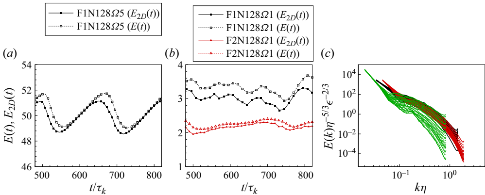
Figure 4. (a) Kinetic energy of the flow field and that in the two-dimensional modes for \Omega = 5 . (b) The same for cases with \Omega = 1 and N = 128 . (c) Instantaneous energy spectra for cases with N = 128 , plotted every 10\tau_k for time spanning 300\tau_k . Green lines indicate \Omega = 5 ; red lines indicate \Omega = 1 with constant power forcing; black lines indicate \Omega = 1 with Kolmogorov forcing.
