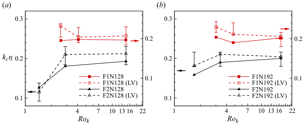
Figure 13. Comparison between the peak wavenumbers for the spectra of the Lyapunov vectors and k_c : (a) cases with N = 128 ; (b) cases with N = 192 . Solid lines and solid symbols indicate k_c \eta (same as figure 10). Dashed lines and empty symbols indicate normalised peak wavenumbers of the spectra of the Lyapunov vectors. Lower groups and left-hand y-axes are for cases with constant power forcing. Upper groups and right-hand y-axes are for cases with Kolmogorov forcing. The error bars correspond to the two adjacent integer wavenumbers.
