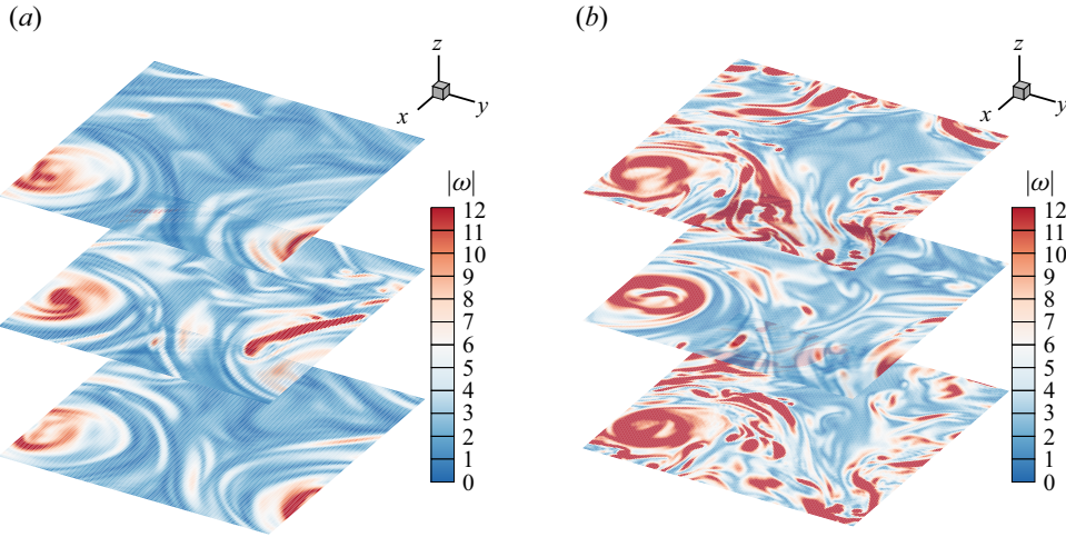
Figure 2. Snapshots of the |\omega| distribution taken at three horizontal layers at the same time t for \Omega = 1 with Kolmogorov forcing: (a) from a case with N = 128 ; (b) from a case with N = 192 .
