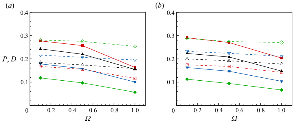
Figure 19. Same as figure 18, but for cases with constant power forcing.
