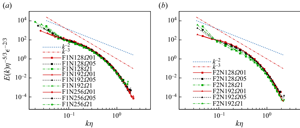
Figure 1. The energy spectra: (a) cases with Kolmogorov forcing; (b) cases with constant power forcing. The dashed line without symbols indicates the k^{-2} power law. The dash-dotted line without symbols indicates the k^{-3} power law.
