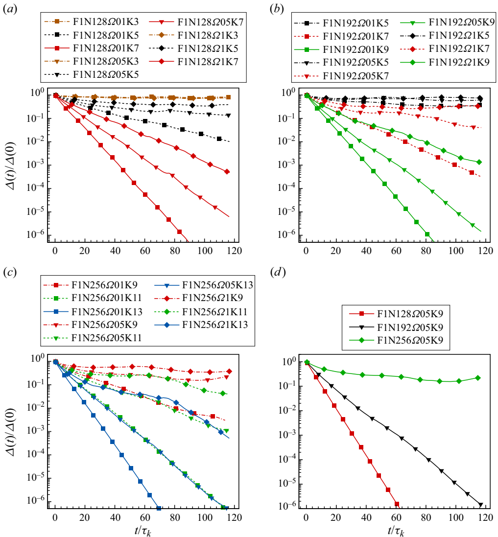
Figure 5. The normalised synchronisation error \Delta(t)/\Delta(0) for the cases with Kolmogorov forcing: (a) N = 128 , (b) N = 192 , (c) N = 256 ; (d) comparison between cases with different Reynolds numbers.
