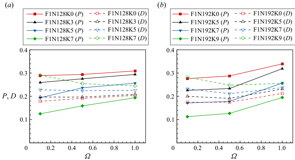
Figure 18. The production term P and the energy dissipation term D for cases with Kolmogorov forcing: (a) N = 128 , (b) N = 192 .
