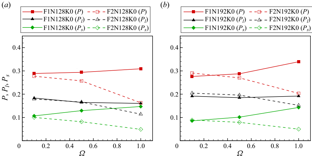
Figure 22. The large-scale ( P_l ) and small-scale ( P_s ) contributions to the production term ( P ): (a) N = 128 , (b) N = 192 .
