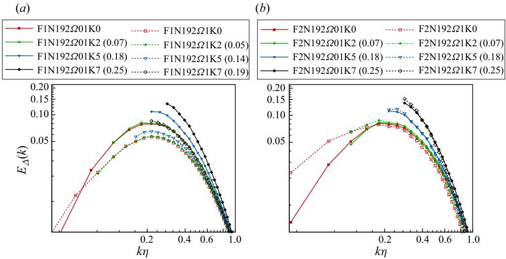
Figure 15. Same as figure 14 but for N = 192 . (a) Cases with Kolmogorov forcing, where k_c\eta = 0.20 for both \Omega = 0.1 and 1 . (b) Cases with constant power forcing, where k_c\eta = 0.20 for \Omega = 0.1 , and k_c\eta = 0.16 for \Omega = 1 .
