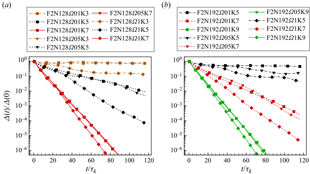
Figure 6. The synchronisation error \Delta(t) for the cases with constant power forcing: (a) N = 128 , (b) N = 192 .
