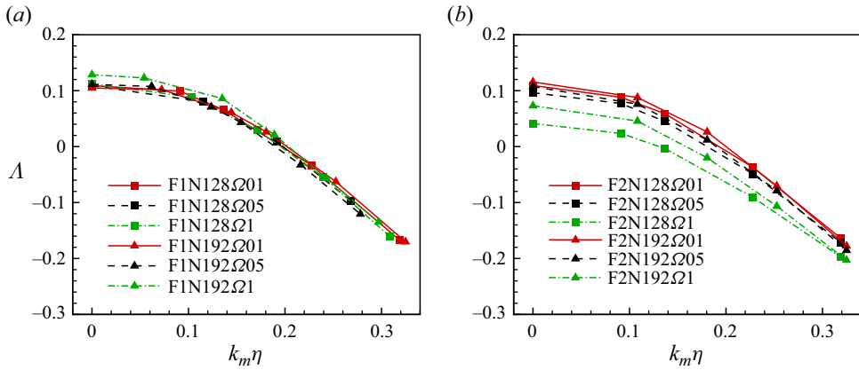
Figure 9. Normalised CLEs \Delta as functions of k_m\eta : (a) cases with Kolmogorov forcing; (b) cases with constant power forcing.
