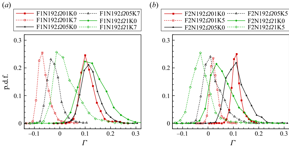
Figure 17. The p.d.f.s of the local Lyapunov exponent \Gamma for selected cases: (a) cases with Kolmogorov forcing; (b) cases with constant power forcing. Note that the p.d.f.s are not normalised.
