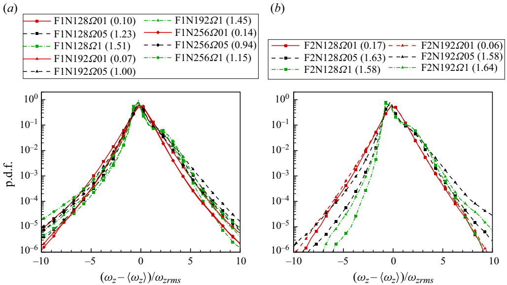
Figure 3. The p.d.f. of the vorticity component along the rotation axis \omega_z : (a) cases with Kolmogorov forcing; (b) cases with constant power forcing.
