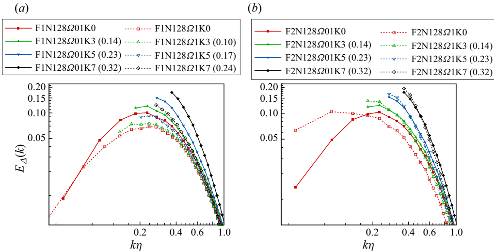
Figure 14. The energy spectra of the conditional Lyapunov vectors \mathbf{u}^\delta for different k_m and N = 128 . The values of k_m\eta are shown in parentheses. (a) Cases with Kolmogorov forcing, where k_c\eta = 0.20 for both \Omega = 0.1 and 1. (b) Cases with constant power forcing, where k_c\eta = 0.19 for \Omega = 0.1 , and k_c\eta = 0.13 for \Omega = 1 .
