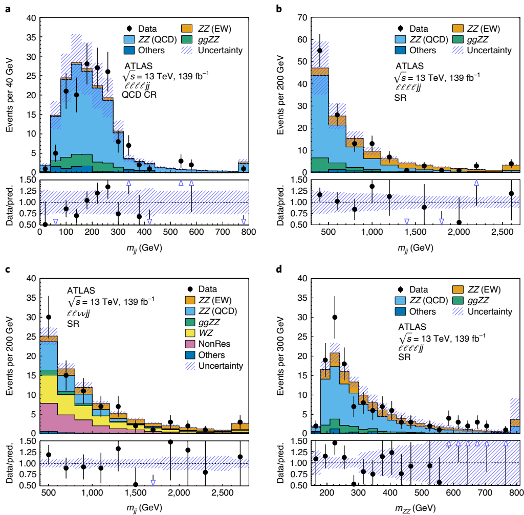
Fig. 2 | Observed and expected distributions. a–d , The m_{ij} distributions in the llllj QCD CR ( a ) and the llllj ( b ) and llvjj SRs ( c ), as well as the m_{zz} distribution in the llllj SR ( d ). The error bands represent the s.d. and include the expected experimental and theoretical systematic uncertainties. The contributions from the QCD and EW production of ZZjj events are scaled by 0.99 and 0.92, respectively, which correspond to the observed normalization factors in the statistical fit to the combined channel (Table 2). ZZ (EW), ZZ (QCD) and ggZZ
