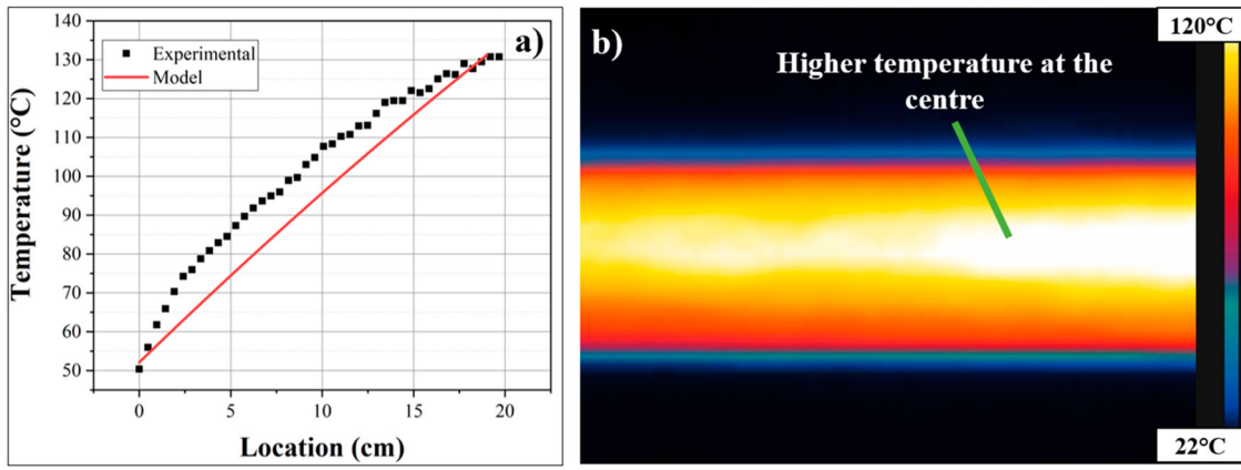
Figure 11. (a) Comparison of predicted temperature values by the model and experimental measurements (b) local temperature variations due to the uneven tension profile across the width of the tape.
