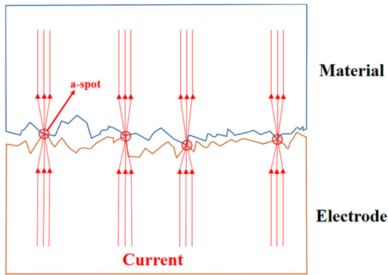
Figure 1. Constrained current flow due to the contact resistances, inspired by Hamedi and Atashparva [33].
