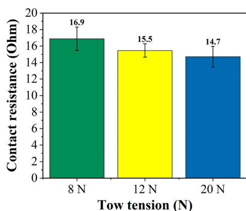
Figure 7. Effect of tow tension on the contact resistances at constant production speed (5 m min -1 ) and room temperature.
