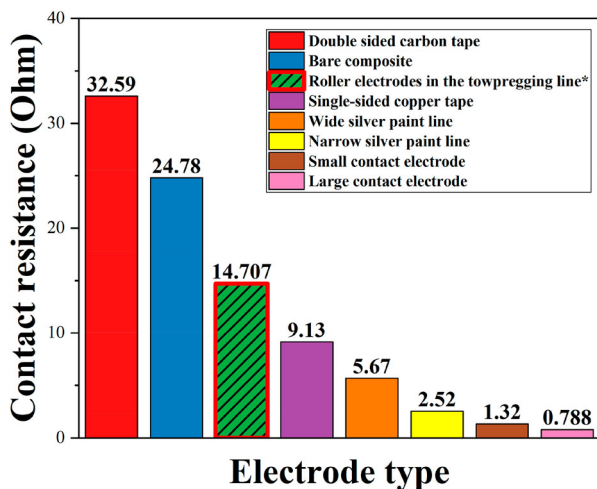
Figure 6. Comparison of contact resistances measured in the towpregging line (at 5 m min -1 production speed and 20 N tension) and different electrode types reported by Kwok and Hahn [9].
