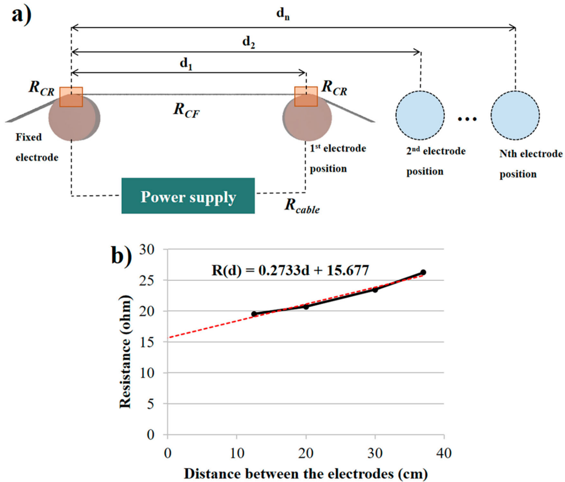
Figure 5. (a) The methodology used to measure the contact resistance of the Joule heating system and (b) sample dataset for linear regression.
