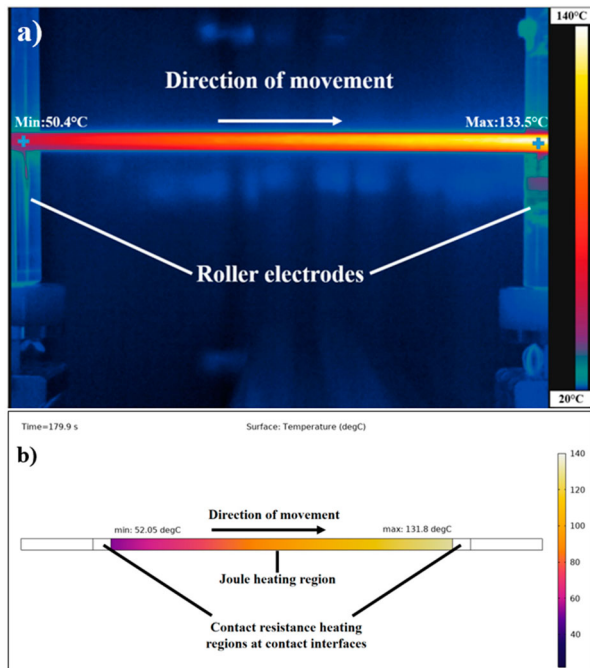
Figure 12. Temperature distribution of the tow captured by IR camera (a) and predicted by the model (b).
