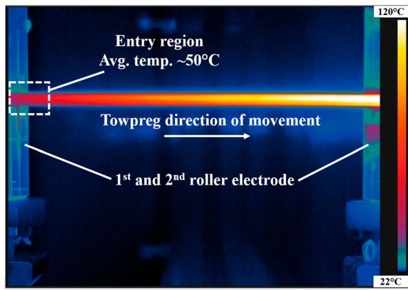
Figure 10. Thermal camera image from the top view of the Joule heating section.
