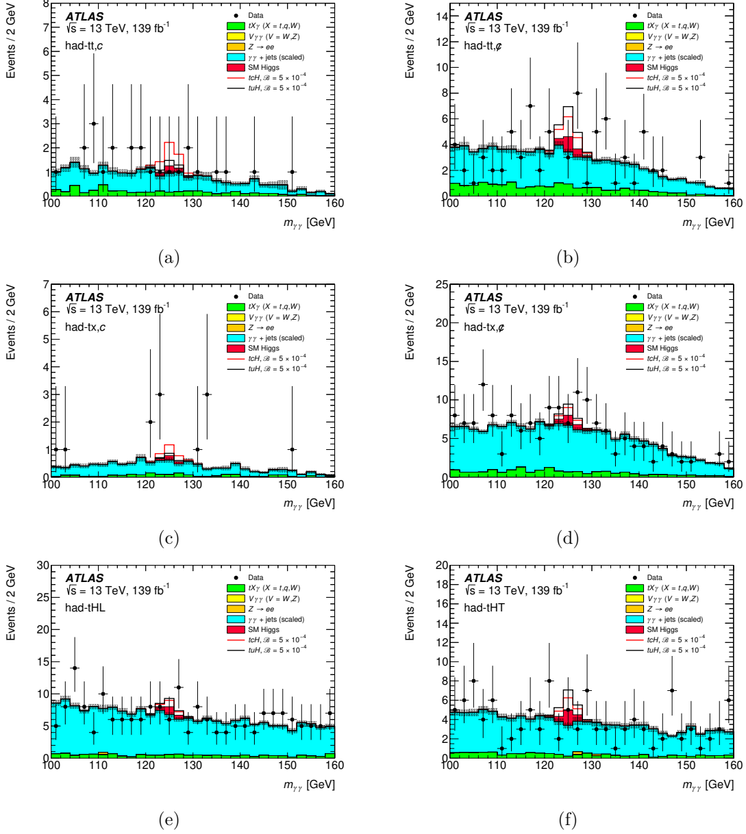
Figure 3. Distributions of the diphoton invariant mass for data, signal, Higgs boson production in the SM, and non-resonant background for the (a) had-tt,c, (b) had-tt, \cancel{e} , (c) had-tx,c, (d) had-tx, \cancel{e} categories after the BDT selection, and (e) had-tHL and (f) had-tHT categories. The hatched bands correspond to the statistical uncertainty in the sum of the simulated non-resonant backgrounds.
