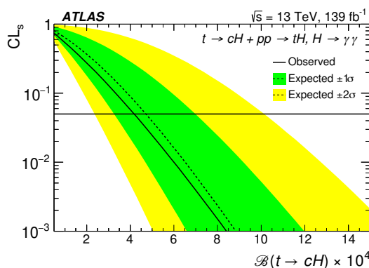
Figure 10. Evolution of the signal confidence level, CL_s , as a function of the t \rightarrow cH branching ratio \mathcal{B} for the observation (full line) and the expectation in the absence of signal (dashed line). The bands at \pm 1\sigma and \pm 2\sigma around the expected curve are also shown.
