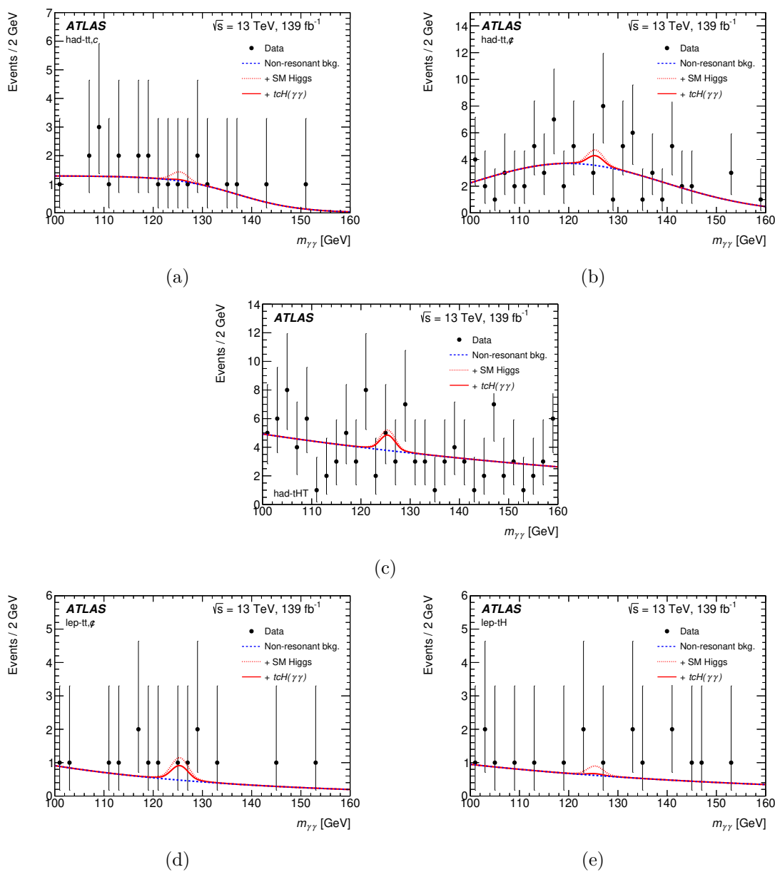
Figure 8. Distributions of the diphoton invariant mass for the most relevant categories: three in the hadronic selection ((a) had-tt,c, (b) had-tt, \phi , and (c) had-tHT) and two in the leptonic selection ((d) lep-tt, \phi and (e) lep-tH). The result of a fit to the data of the sum (full line) of a signal component with the mass of the Higgs boson fixed to m_H = 125 \text{ GeV} and assuming a non-zero tcH coupling, a non-resonant background component (dashed line) and the SM Higgs boson contribution (difference between the dotted and dashed lines) is superimposed.
