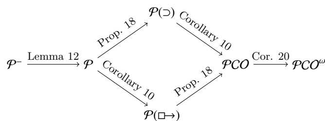
■ Figure 1 Arrows denote strict inclusion of expressivity; \mathcal{P}(\Box\rightarrow) and \mathcal{P}(\supset) are incomparable.
