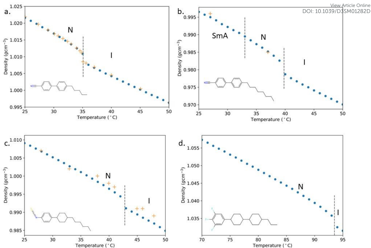
Figure 4. Densities of the liquid crystal materials at 1°C intervals. Dashed lines denote transition temperatures as defined by the temperature of the largest density gradient. The density increases at the phase transition are readily observable for the I-N transitions, but more subtle for the N-SmA transition. Comparison is made with literature data where possible (orange plus points) for (a) 5CB [30], (b) 8CB [35] and (c) (NCS)PCH6 [37]. (d) The CCU-3-F figure is representative of the scarcity of LC density data.
