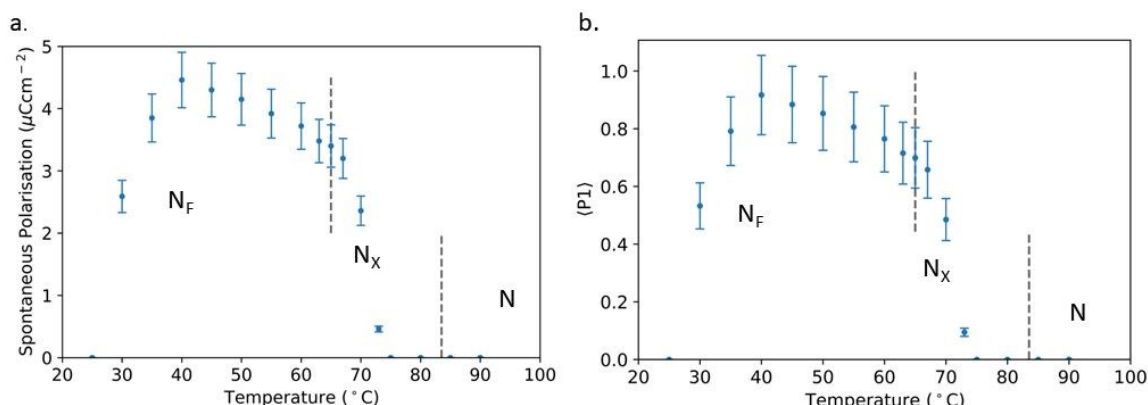
Figure 8. a) Spontaneous polarisation measurements of DIO (see Fig. 1 for DIO's structure and phase sequence) on cooling through its N_F - N_X - N phase sequence until crystallisation. Switching current response peaks are integrated to give the magnitude of polarisation. b) An approximation of \langle P1 \rangle for DIO from the contribution of average molecular dipole alignment to the polarisation.
