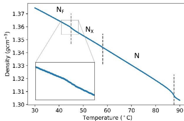
Figure 5. Temperature-dependent density behaviour for the N_F material M5 across its phase range. The initial increase with first nematic ordering is on cooling from the isotropic phase at 87.6^\circ\text{C} similar to the other selected materials. There is no discernible change in density at the N-N_X phase transition. There is a small increase at 45^\circ\text{C} that can be attributed to the effects of polar ordering. The high average density of M5 should also be noted. Inset: N_X-N_F transition
