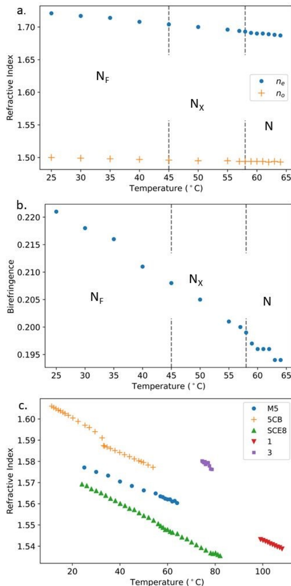
Figure 7. a) The n_o and n_e measurements of M5 at 589nm as the sample is cooled through its N-N X -N F phase sequence. b) The resulting birefringence ( \Delta n = n_e - n_o ) values of M5. c) A comparison is made of n_{avg} for M5 and 5CB [42] as well as the polar smectics, SCE8 [43] and compounds 1 and 3 from [44, 45].
