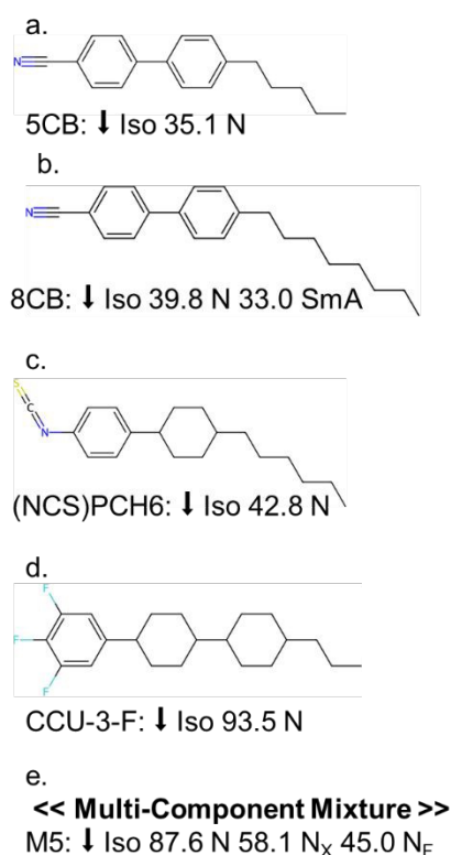
Figure 3. Chemical structures of the materials for which density measurements were undertaken. Transition temperatures ( T , °C) on cooling (↓) were determined from density measurements and are in good agreement with DSC data (SI section S1). For single component materials (a-d) molecular structures are given.
