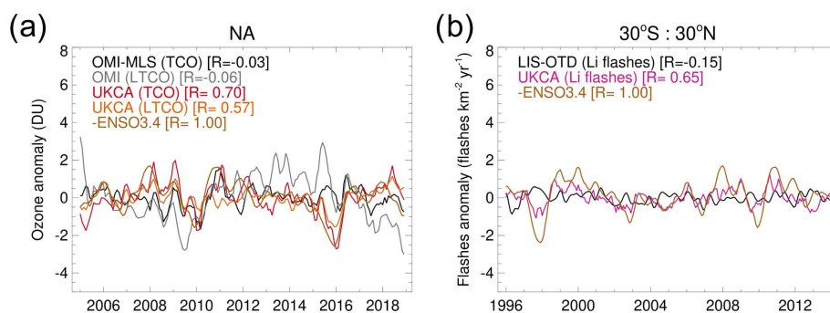
Figure 11. Deseasonalized and detrended time series anomalies of ( a ) observed and modelled ozone in the North Atlantic and ( b ) tropical lightning flashes. The - ENSO index time series is also plotted for comparison. Correlation coefficients ( R ) between each time series and the - ENSO index are noted in the legends.
