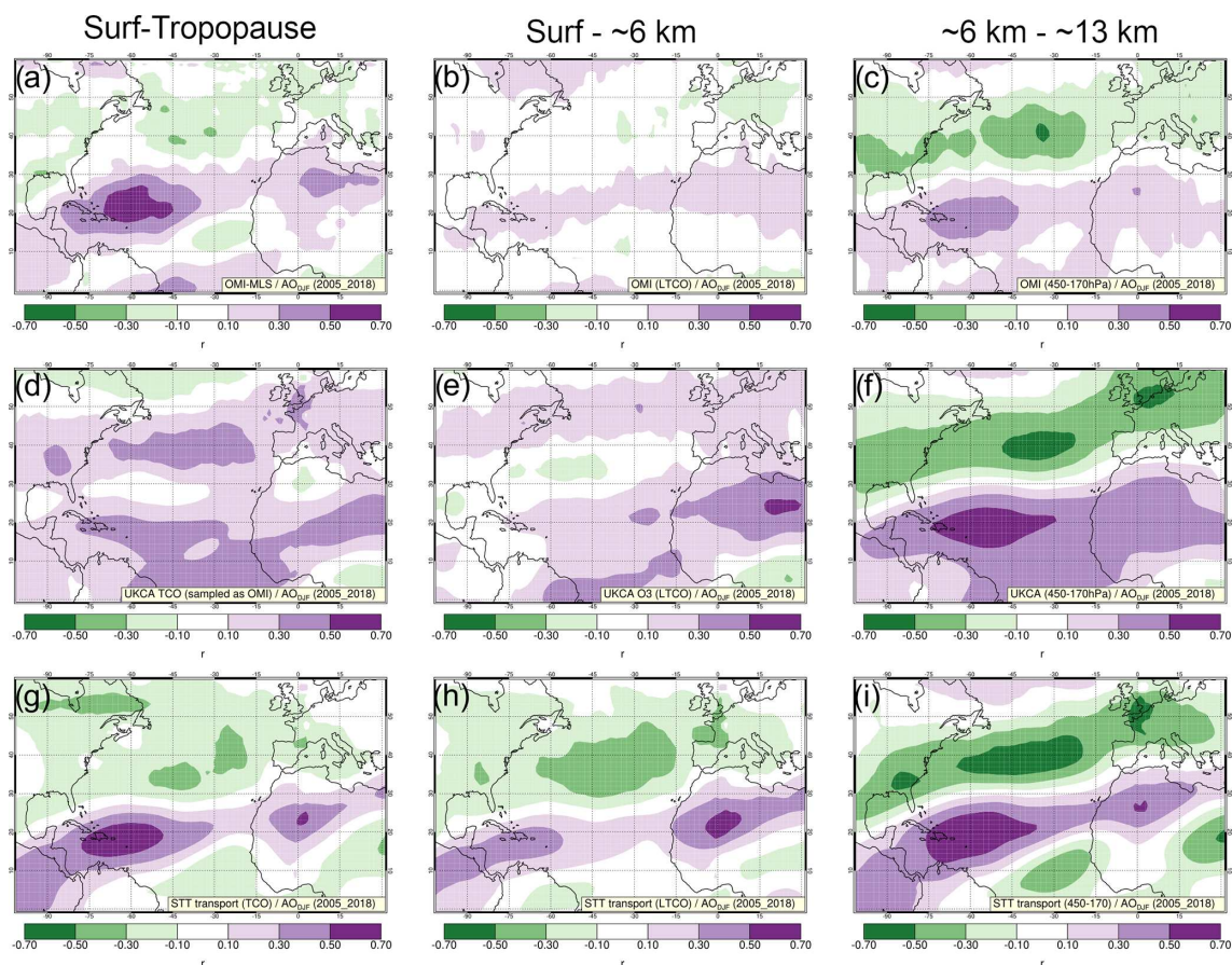
Figure 10. Correlation maps between the AO (in DJF) and observed ozone ( a, b, c ), modelled ozone ( d, e, f ) and modelled stratosphere to troposphere transport ( g, h, i ). The first column shows correlation for variables integrated over the full troposphere (surface to tropopause), while the second and third columns show correlation for variables integrated over the OMI subcolumns: surface–450 hPa ( \sim 0 –6 km) and 450–170 hPa ( \sim 6 –13 km).
