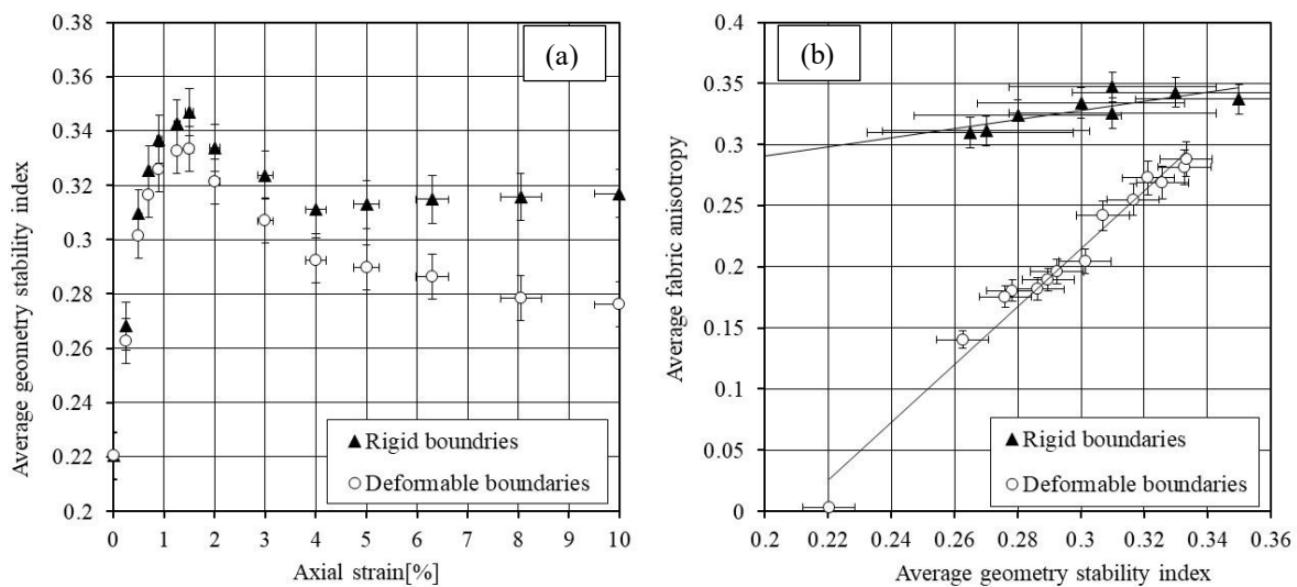
15 16 Figure 11 (a) The sensitivity of average geometrical stability index to the different boundary condition, linear 17 coloration between average fabric anisotropy and average geometrical stability index
