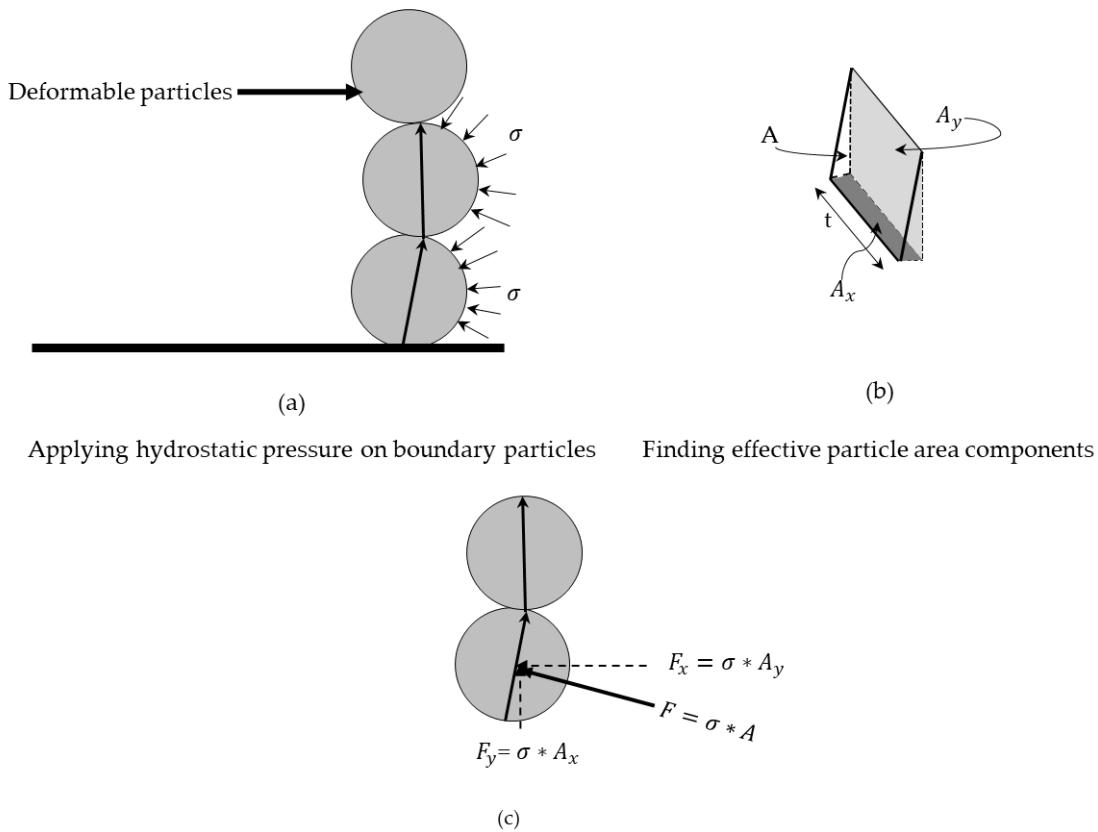
Applying hydrostatic forces on boundary particles
