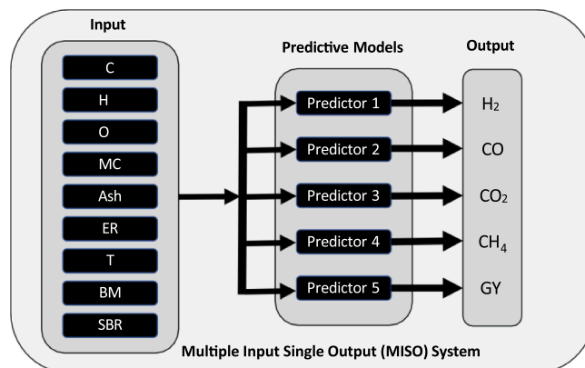
Fig. 1. Multiple Input and Single Output (MISO) systems and Data descriptor: input variables x = [C, H, O, MC, \text{Ash}, ER, T, BM, \text{SBR}] and output variables y = [H_2, CO, CO_2, CH_4, GY] , where carbon (C), hydrogen (H), oxygen (O), moisture (MC) and ash (Ash) contents for the biomass, and the process parameters such as equivalence ratio (ER), reactor temperature (T), bed material (BM), steam to biomass mass ratio (SBR), hydrogen (H 2 ), carbon monoxide (CO), carbon dioxide (CO 2 ), methane (CH 4 ), and gas yield (GY). MISO uses all nine input variables to estimate the composition of each output composition by training five different prediction models (i.e. Predictor 1 to Predictor 5).
