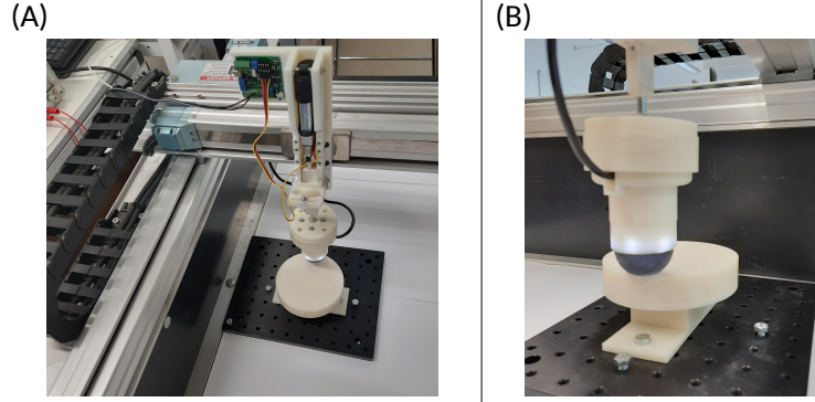
Fig. 1. Robotic setting. A) The Robotic platform consists of a Yamaha "XYX" robot and an Actuatorix P-16 linear actuator vertical displacements. B) TacTip sensor [3] with the stimulus for data collection
