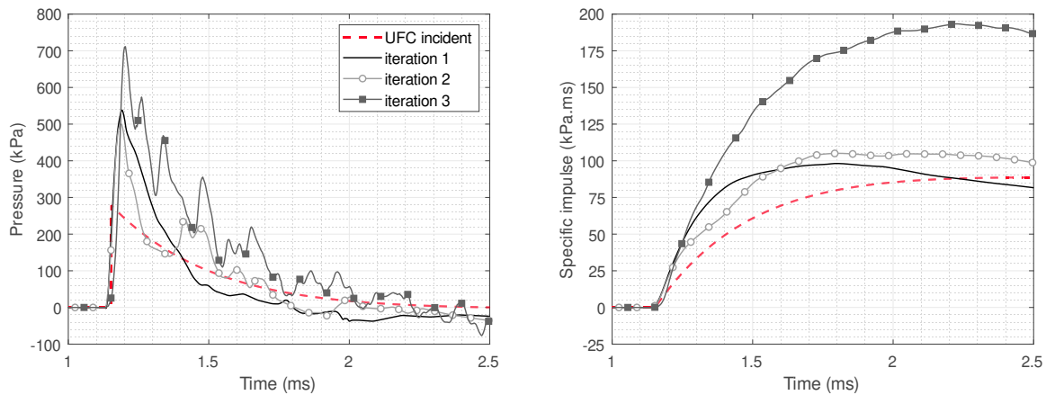
Figure 7. “On-obstacle” reflected pressure and specific impulse histories (S12; 1.35 m slant distance from a 250 g PE4 hemisphere). UFC incident predictions shown in red.
