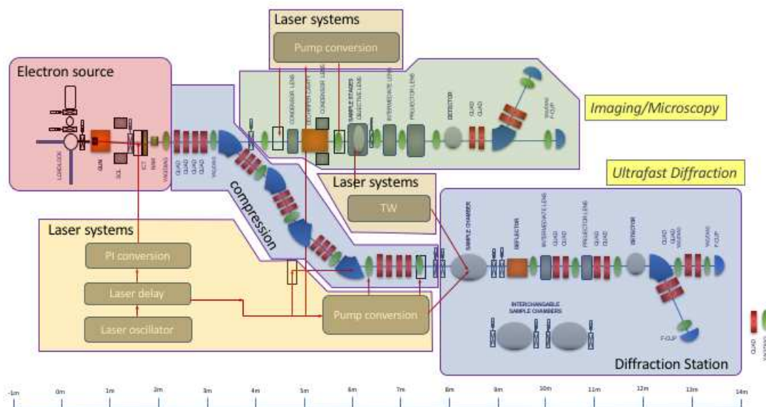
Figure 1: Working concept for the configuration of RUEDI system with diffraction and Imaging line.
