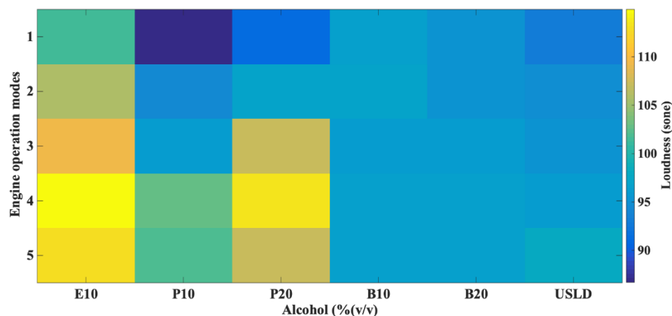
Figure 9. Loudness for alcohol diesel fuel blends; 10% ( v/v ) ethanol/diesel fuel (E10), 10% ( v/v ) propanol/diesel fuel (P10), 20% ( v/v ) propanol/diesel fuel (P20), 10% ( v/v ) butanol/diesel fuel (B10), 20% ( v/v ) butanol/diesel fuel (B20) and 100% ultra-low -sulfur diesel fuel (USLD).
