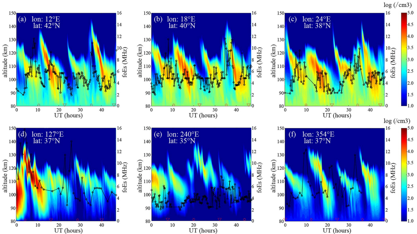
Figure 2. The temporal variations of simulated \text{Fe}^+ density and observed foEs (Es critical frequency) over six mid-latitude stations during 10–11 July 2007. The Es layer model is driven by neutral winds from High Altitude Mechanistic General Circulation Model with total waves (horizontal wavelength larger than \sim 156 km). The black solid lines represent the foEs recorded by ionosondes. The simulations were run for 72 hr and the first 24 hr were discarded. \circ and \nabla on the horizontal axis represent the local noon (12:00 LT) and local midnight (24:00 LT), respectively.
