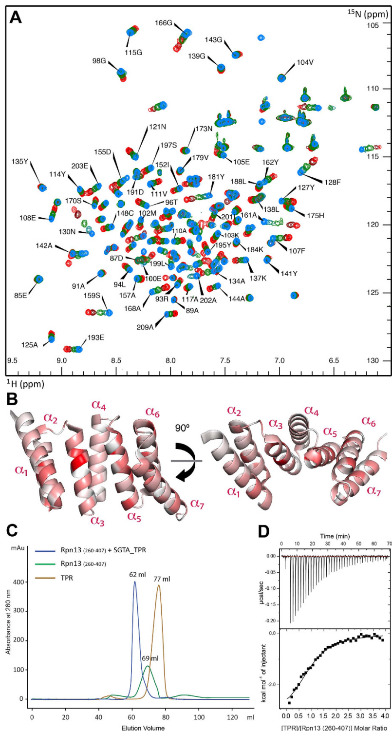
Figure 1. SGTA_TPR/Rpn13 260-407 interaction studies. (A) 1 H- 15 N HSQC spectra of 15 N-labelled SGTA_TPR at different titration points with unlabelled Rpn13 260-407 (1:0, 1:1, 1:2, 1:3, 1:8; in blue, teal, green, maroon, and red respectively). (B) Orthogonal cartoon views of SGTA_TPR (PDB accession code 2VYI) 18 coloured according to normalised chemical shift perturbation (CSP) \Delta\delta^{av} values upon binding to Rpn13 260-407 with most perturbed residues shown in red. (C) Size exclusion chromatography (SEC) experiments showing the formation of a stable complex as evident by co-elution of SGTA_TPR with Rpn13 260-407 . (D) ITC data showing binding of SGTA_TPR to Rpn13 260-407 . The thermodynamic binding constant of this interaction as determined by ITC was, K_d = 16.1 \pm 1.4 \mu\text{M} .
