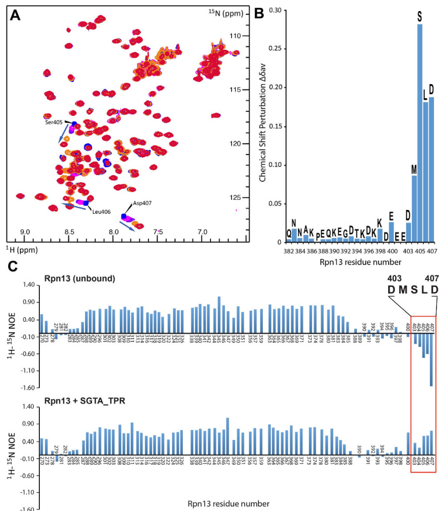
Figure 2. The extreme C-terminus of Rpn13 260-407 is the SGTA_TPR interacting region. (A) ^1\text{H} - ^{15}\text{N} HSQC spectra of ^{15}\text{N} -labelled Rpn13 260-407 at different titration points with unlabelled SGTA_TPR (1:0, 1:0.2, 1:0.5, 1:0.7, 1:1; in blue, light green, green, maroon, and red respectively). (B) Chemical shift perturbation (CSP) \Delta\delta^{\text{av}} values derived from (A) of Rpn13 C-terminal residues 382–407 upon binding to SGTA_TPR. (C) ^1\text{H} - ^{15}\text{N} heteronuclear NOE enhancement values of Rpn13 C-terminal residues in unbound and SGTA_TPR bound states.
